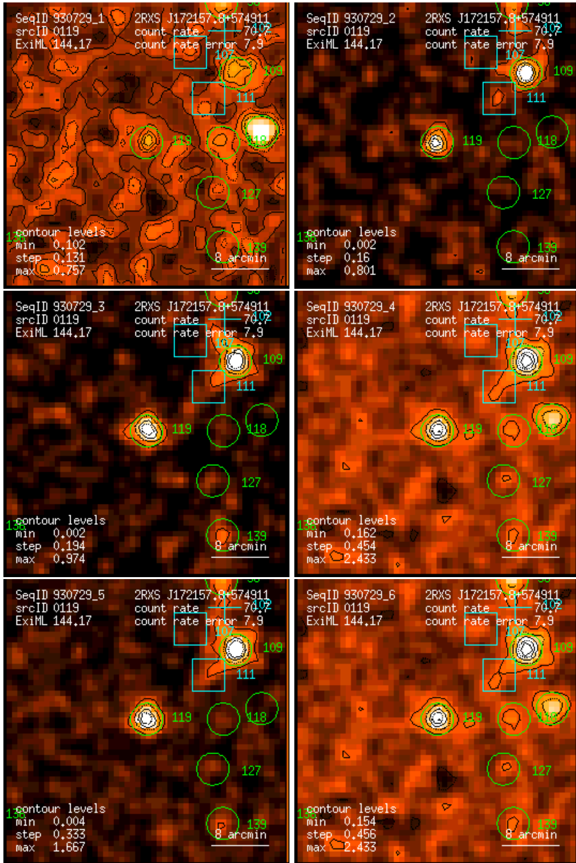
Figure 119: RASS 930729: detection 0119: band rate images, Gaussian filter: (1) PSPC channels 11 – 41, (2) 52 – 90, (3) 91 – 201, (4) 11 – 235, (5) 52 – 201, (6) 11 – 201. Broad band rates in counts/ks. Band rate contour levels in counts/ks/arcmin 2 .
