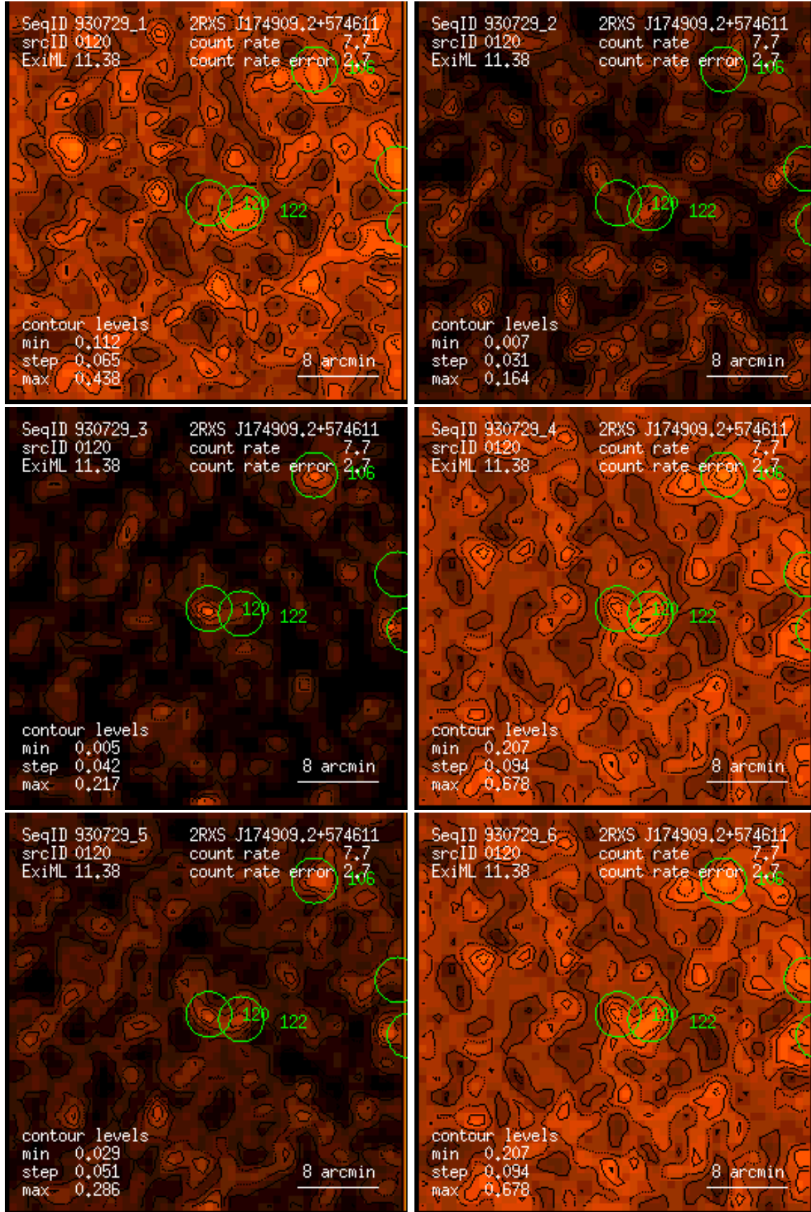
Figure 120: RASS 930729: detection 0120: band rate images, Gaussian filter: (1) PSPC channels 11 – 41, (2) 52 – 90, (3) 91 – 201, (4) 11 – 235, (5) 52 – 201, (6) 11 – 201. Broad band rates in counts/ks. Band rate contour levels in counts/ks/arcmin 2 .
