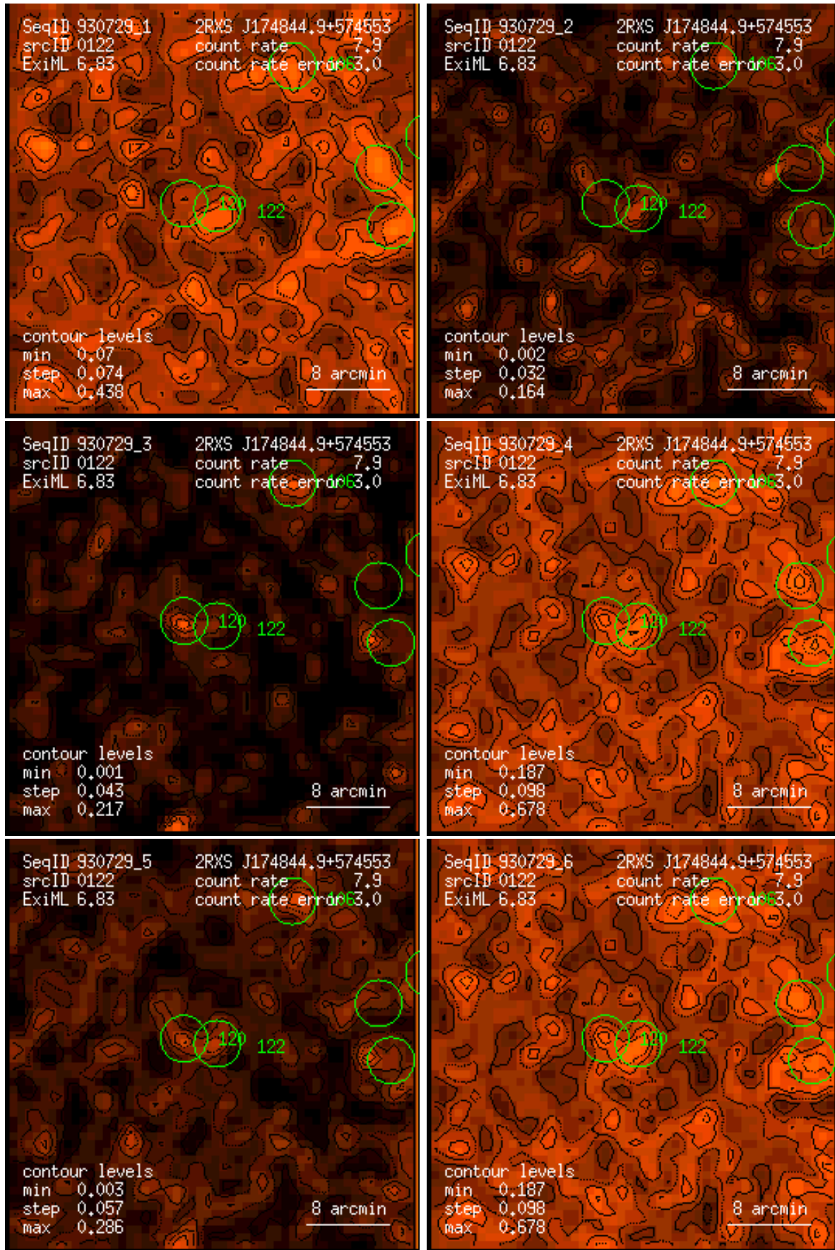
Figure 122: RASS 930729: detection 0122: band rate images, Gaussian filter: (1) PSPC channels 11 – 41, (2) 52 – 90, (3) 91 – 201, (4) 11 – 235, (5) 52 – 201, (6) 11 – 201. Broad band rates in counts/ks. Band rate contour levels in counts/ks/arcmin 2 .
