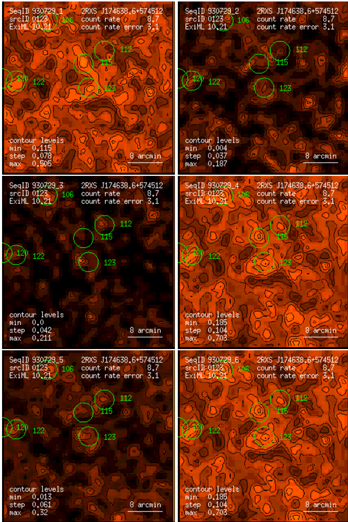
Figure 123: RASS 930729: detection 0123: band rate images, Gaussian filter: (1) PSPC channels 11 – 41, (2) 52 – 90, (3) 91 – 201, (4) 11 – 235, (5) 52 – 201, (6) 11 – 201. Broad band rates in counts/ks. Band rate contour levels in counts/ks/arcmin 2 .
