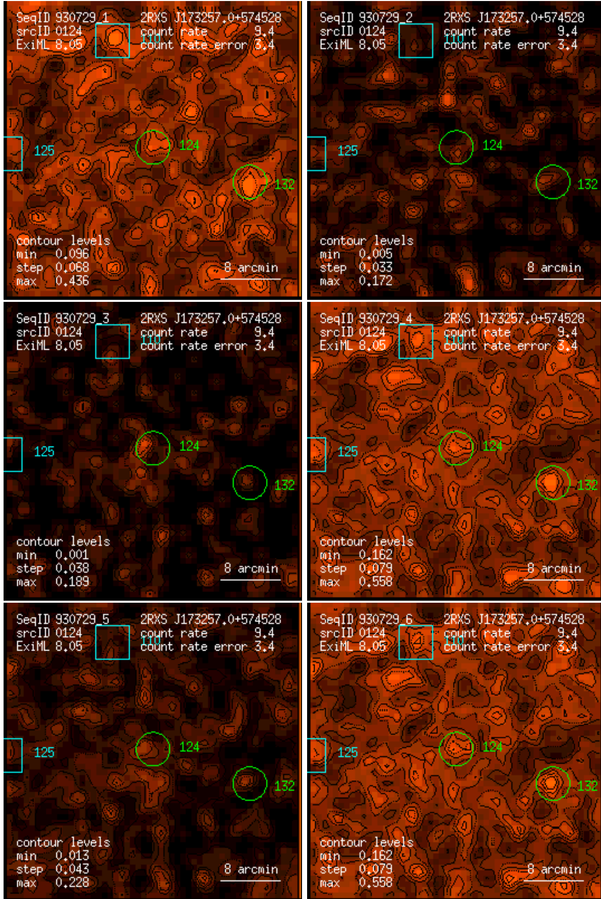
Figure 124: RASS 930729: detection 0124: band rate images, Gaussian filter: (1) PSPC channels 11 – 41, (2) 52 – 90, (3) 91 – 201, (4) 11 – 235, (5) 52 – 201, (6) 11 – 201. Broad band rates in counts/ks. Band rate contour levels in counts/ks/arcmin 2 .
