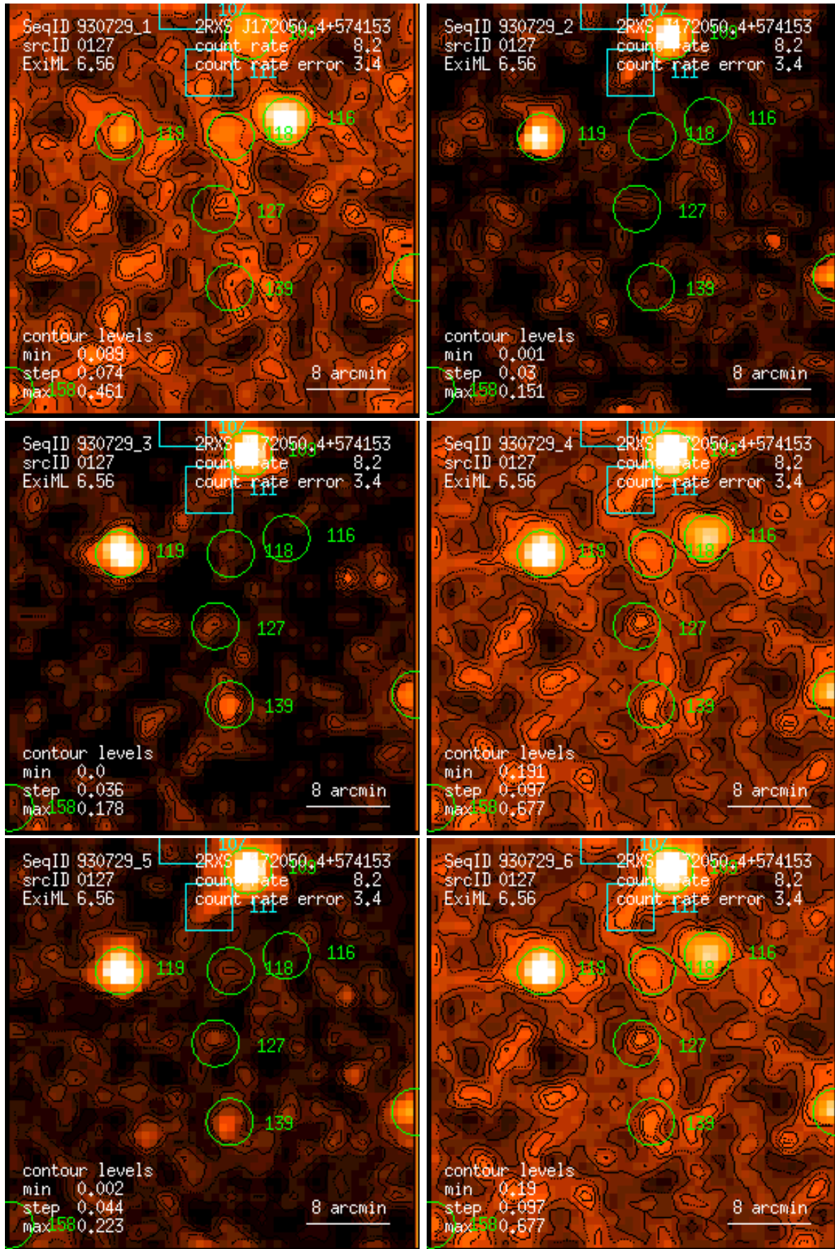
Figure 127: RASS 930729: detection 0127: band rate images, Gaussian filter: (1) PSPC channels 11 – 41, (2) 52 – 90, (3) 91 – 201, (4) 11 – 235, (5) 52 – 201, (6) 11 – 201. Broad band rates in counts/ks. Band rate contour levels in counts/ks/arcmin 2 .
