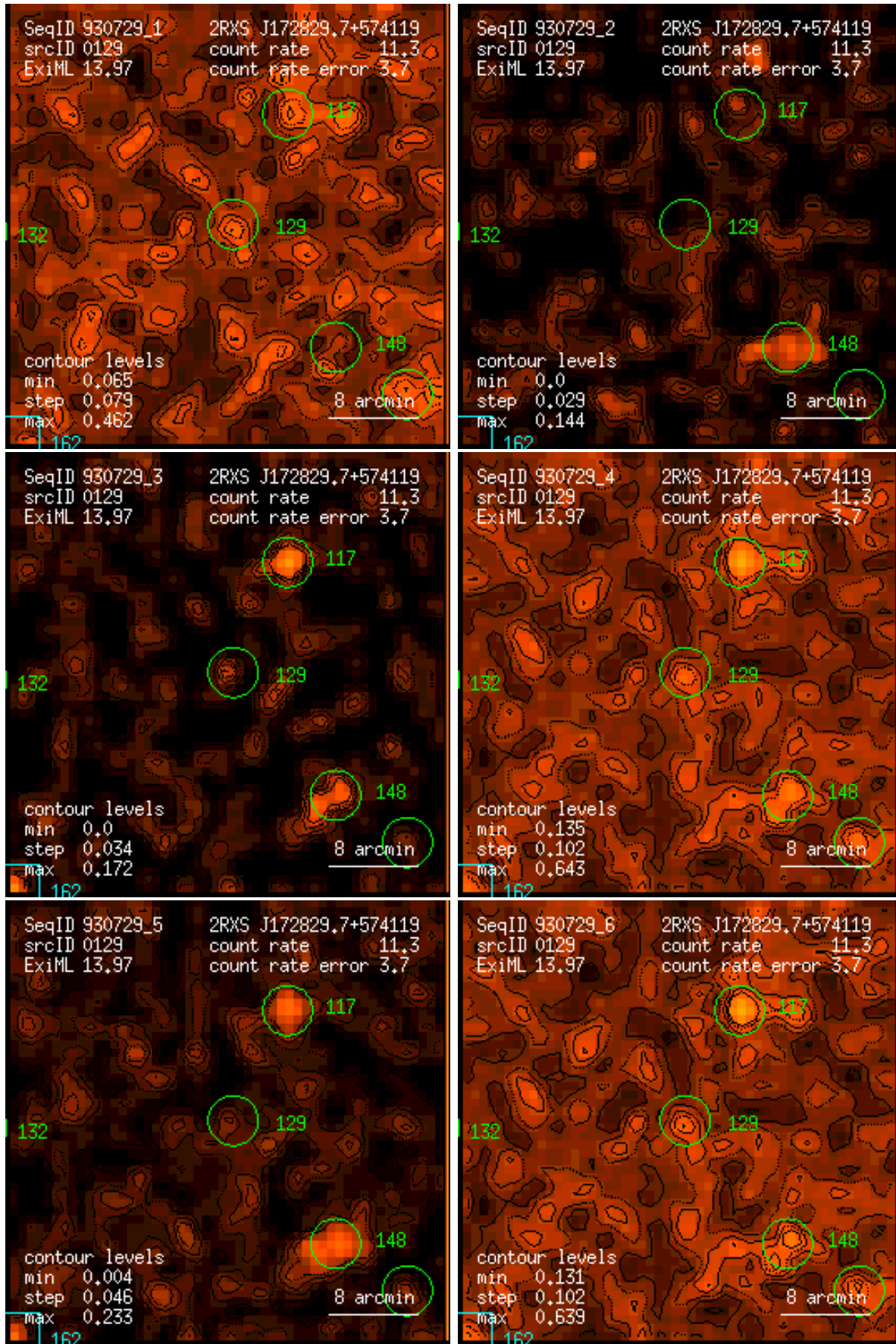
Figure 129: RASS 930729: detection 0129: band rate images, Gaussian filter: (1) PSPC channels 11 – 41, (2) 52 – 90, (3) 91 – 201, (4) 11 – 235, (5) 52 – 201, (6) 11 – 201. Broad band rates in counts/ks. Band rate contour levels in counts/ks/arcmin 2 .
