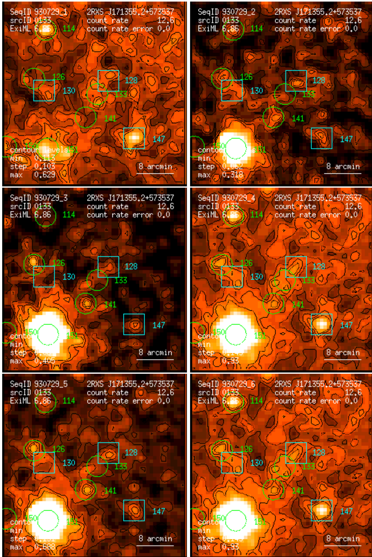
Figure 133: RASS 930729: detection 0133: band rate images, Gaussian filter: (1) PSPC channels 11 – 41, (2) 52 – 90, (3) 91 – 201, (4) 11 – 235, (5) 52 – 201, (6) 11 – 201. Broad band rates in counts/ks. Band rate contour levels in counts/ks/arcmin 2 .
