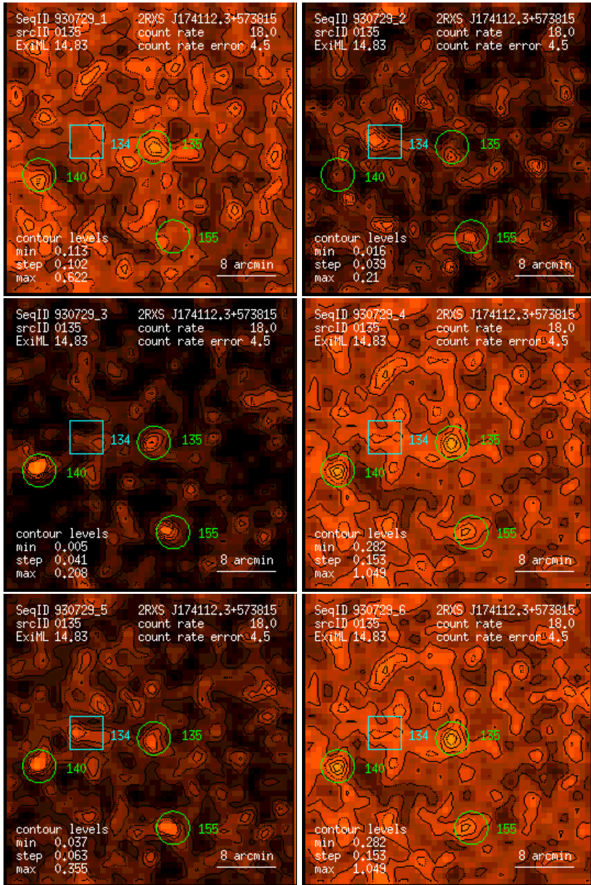
Figure 135: RASS 930729: detection 0135: band rate images, Gaussian filter: (1) PSPC channels 11 – 41, (2) 52 – 90, (3) 91 – 201, (4) 11 – 235, (5) 52 – 201, (6) 11 – 201. Broad band rates in counts/ks. Band rate contour levels in counts/ks/arcmin 2 .
