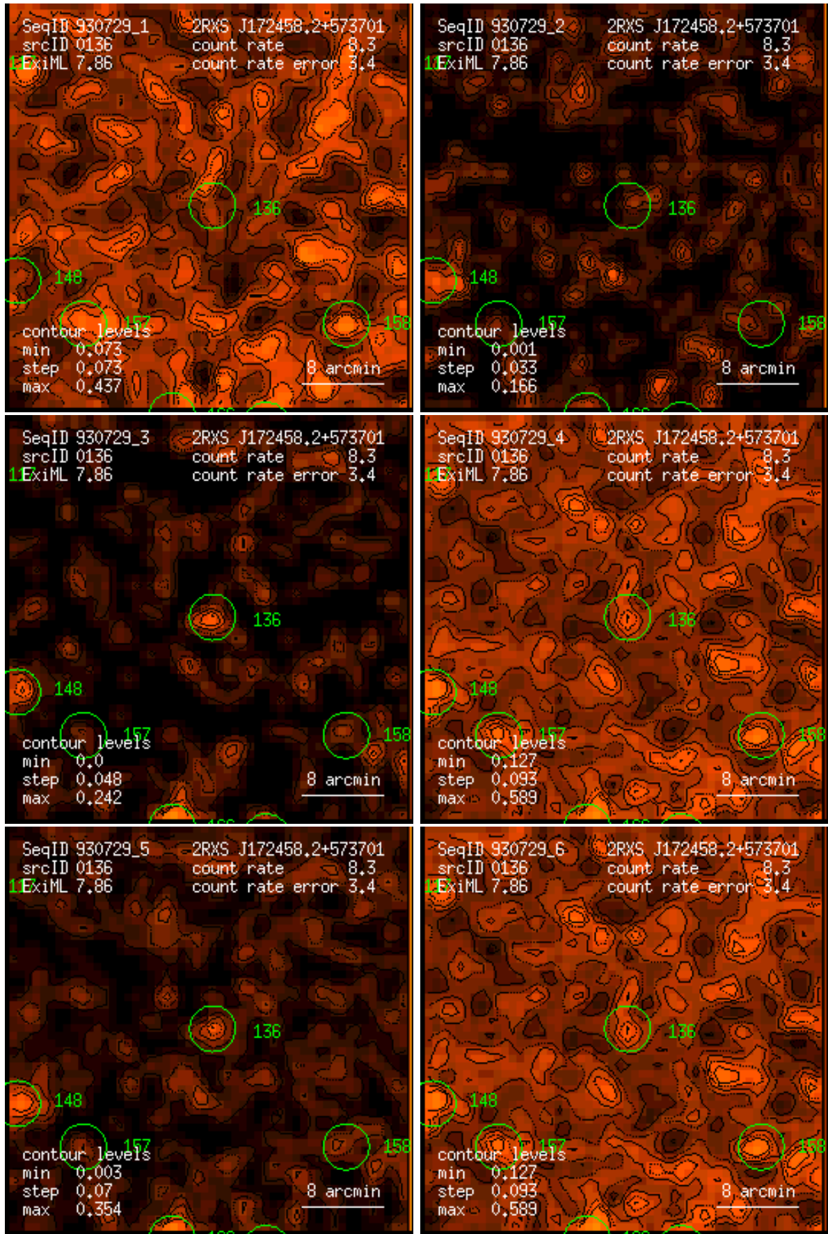
Figure 136: RASS 930729: detection 0136: band rate images, Gaussian filter: (1) PSPC channels 11 – 41, (2) 52 – 90, (3) 91 – 201, (4) 11 – 235, (5) 52 – 201, (6) 11 – 201. Broad band rates in counts/ks. Band rate contour levels in counts/ks/arcmin 2 .
