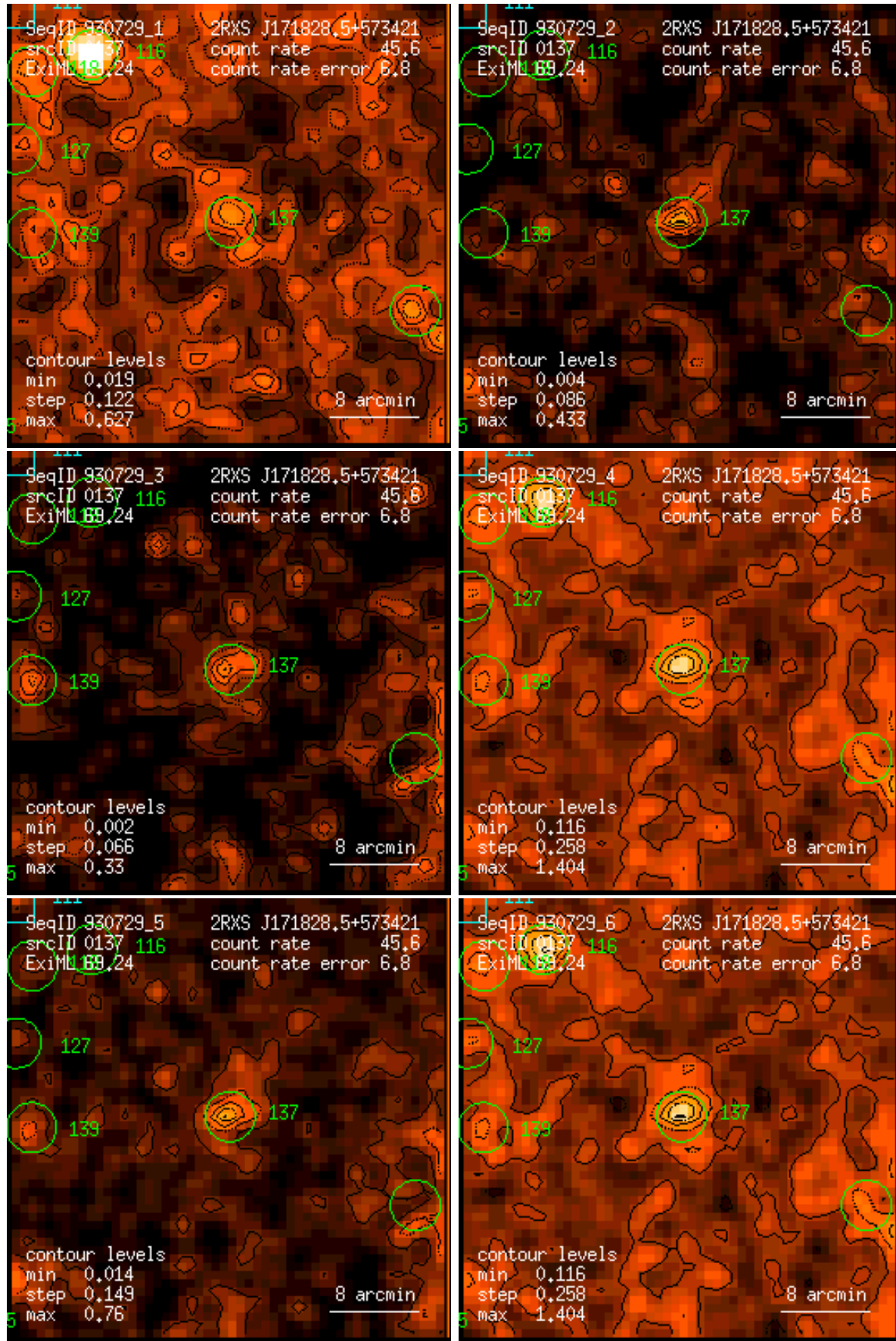
Figure 137: RASS 930729: detection 0137: band rate images, Gaussian filter: (1) PSPC channels 11 – 41, (2) 52 – 90, (3) 91 – 201, (4) 11 – 235, (5) 52 – 201, (6) 11 – 201. Broad band rates in counts/ks. Band rate contour levels in counts/ks/arcmin 2 .
