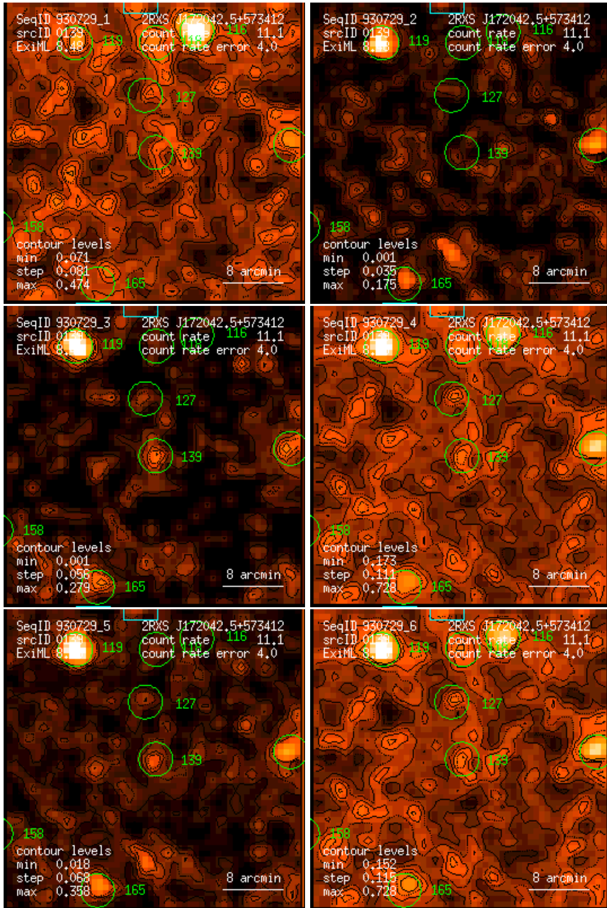
Figure 139: RASS 930729: detection 0139: band rate images, Gaussian filter: (1) PSPC channels 11 – 41, (2) 52 – 90, (3) 91 – 201, (4) 11 – 235, (5) 52 – 201, (6) 11 – 201. Broad band rates in counts/ks. Band rate contour levels in counts/ks/arcmin 2 .
