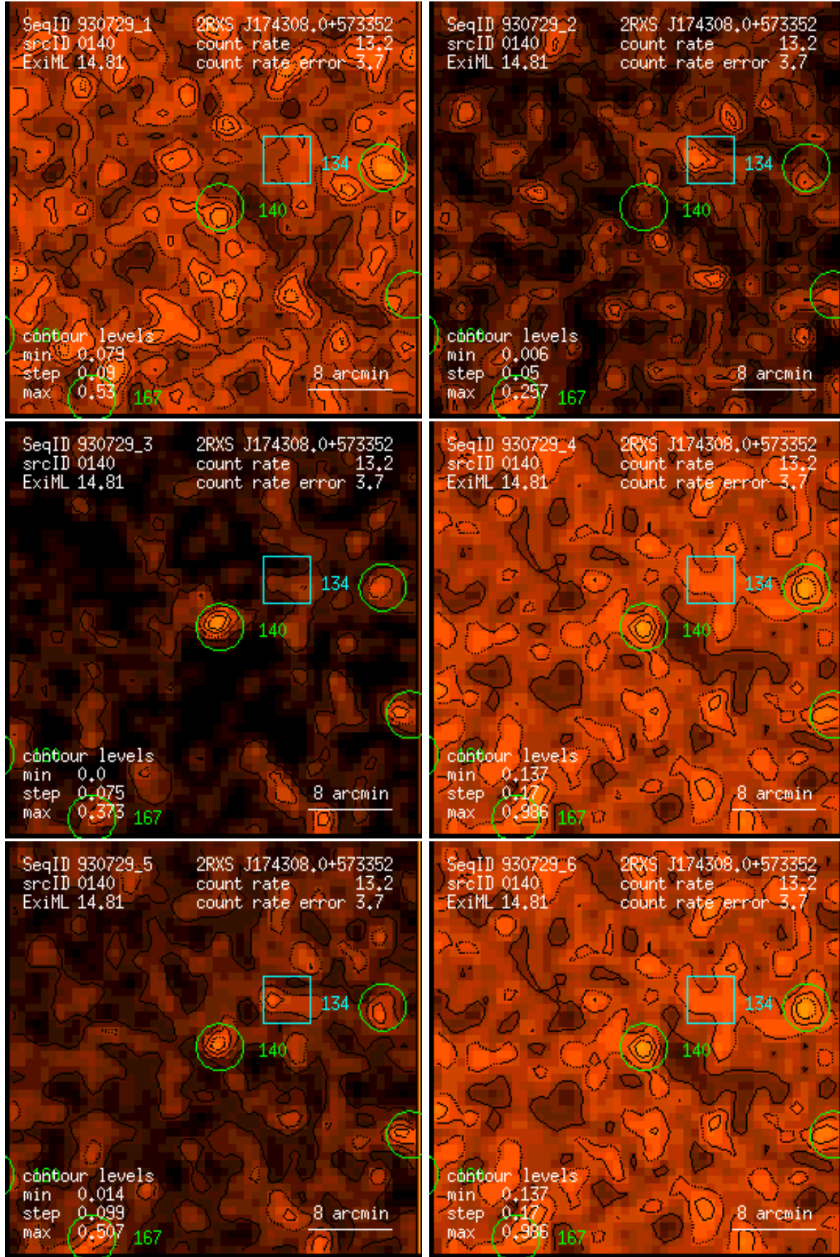
Figure 140: RASS 930729: detection 0140: band rate images, Gaussian filter: (1) PSPC channels 11 – 41, (2) 52 – 90, (3) 91 – 201, (4) 11 – 235, (5) 52 – 201, (6) 11 – 201. Broad band rates in counts/ks. Band rate contour levels in counts/ks/arcmin 2 .
