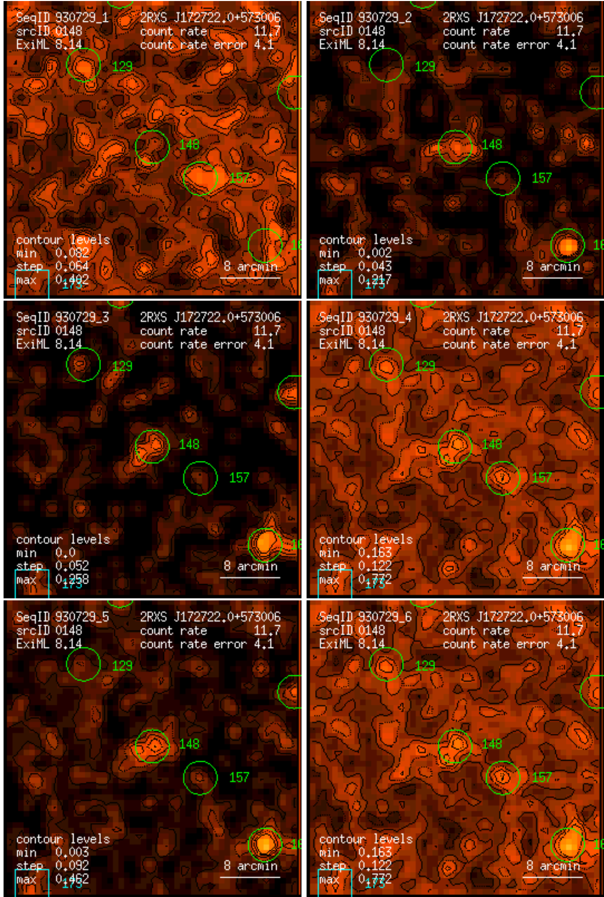
Figure 148: RASS 930729: detection 0148: band rate images, Gaussian filter: (1) PSPC channels 11 – 41, (2) 52 – 90, (3) 91 – 201, (4) 11 – 235, (5) 52 – 201, (6) 11 – 201. Broad band rates in counts/ks. Band rate contour levels in counts/ks/arcmin 2 .
