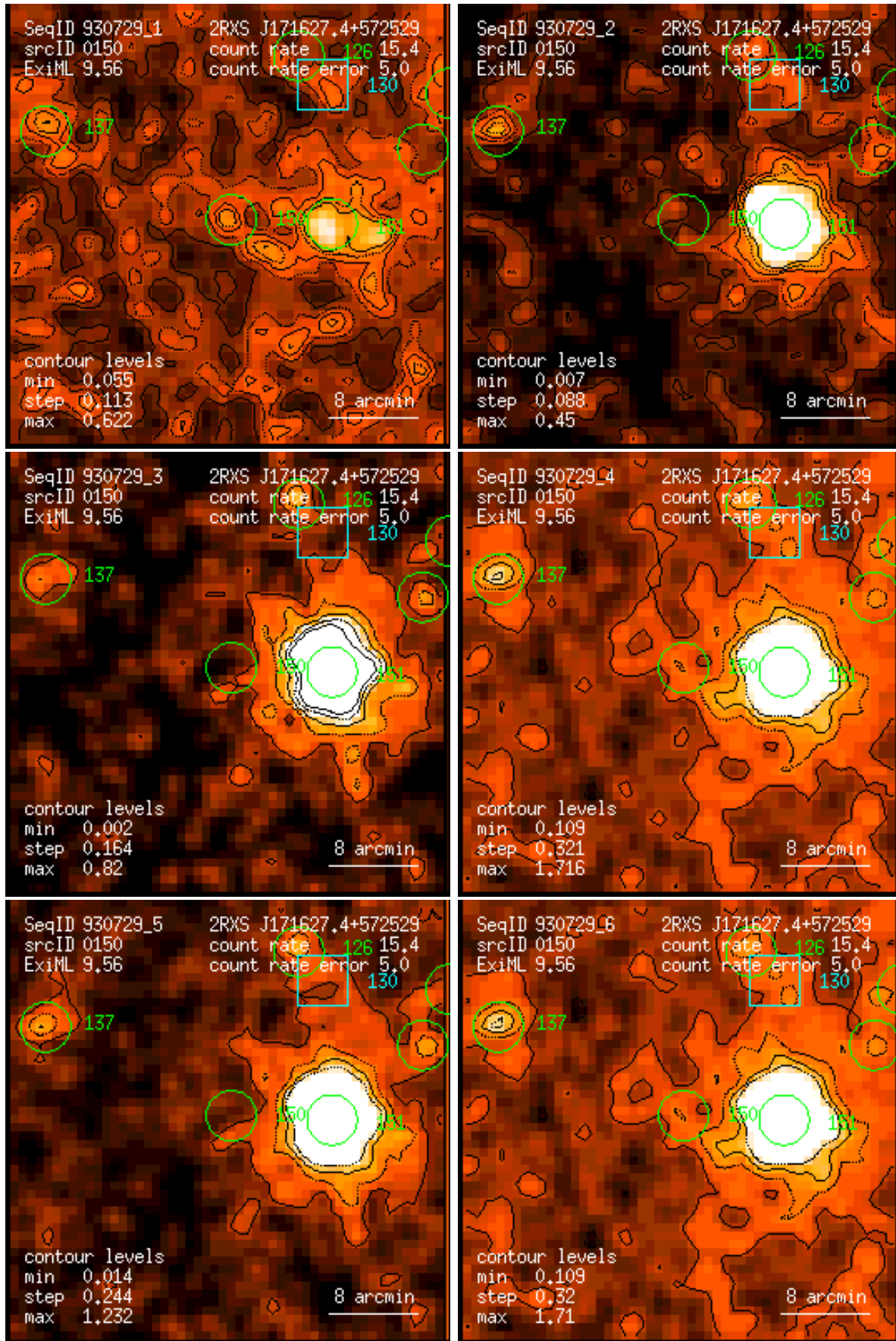
Figure 150: RASS 930729: detection 0150: band rate images, Gaussian filter: (1) PSPC channels 11 – 41, (2) 52 – 90, (3) 91 – 201, (4) 11 – 235, (5) 52 – 201, (6) 11 – 201. Broad band rates in counts/ks. Band rate contour levels in counts/ks/arcmin 2 .
