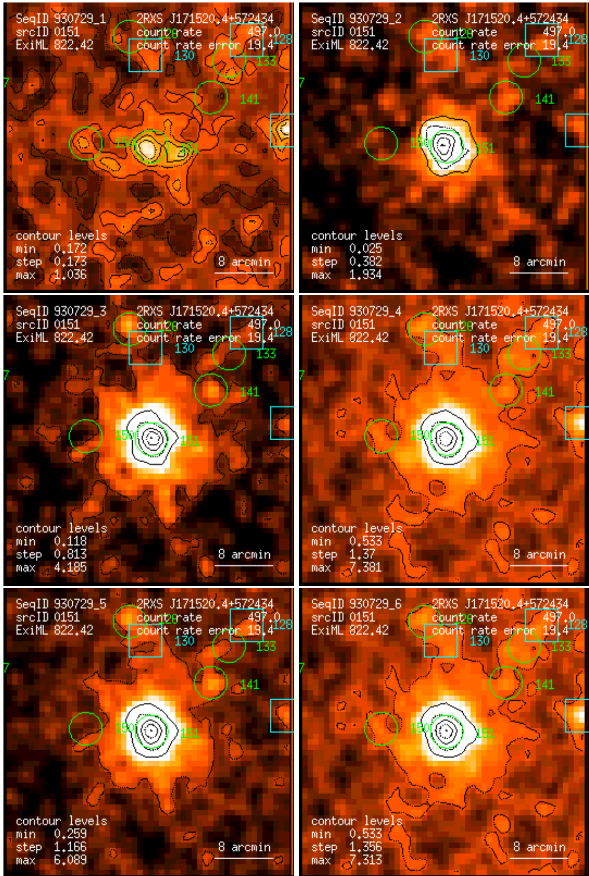
Figure 151: RASS 930729: detection 0151: band rate images, Gaussian filter: (1) PSPC channels 11 – 41, (2) 52 – 90, (3) 91 – 201, (4) 11 – 235, (5) 52 – 201, (6) 11 – 201. Broad band rates in counts/ks. Band rate contour levels in counts/ks/arcmin 2 .
