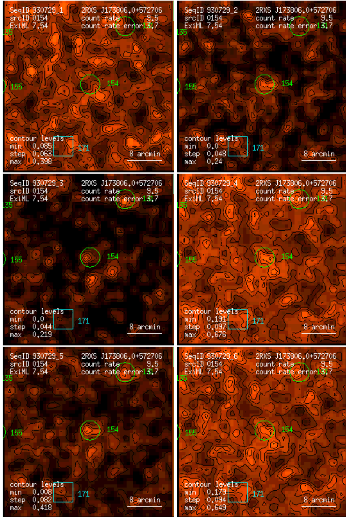
Figure 154: RASS 930729: detection 0154: band rate images, Gaussian filter: (1) PSPC channels 11 – 41, (2) 52 – 90, (3) 91 – 201, (4) 11 – 235, (5) 52 – 201, (6) 11 – 201. Broad band rates in counts/ks. Band rate contour levels in counts/ks/arcmin 2 .
