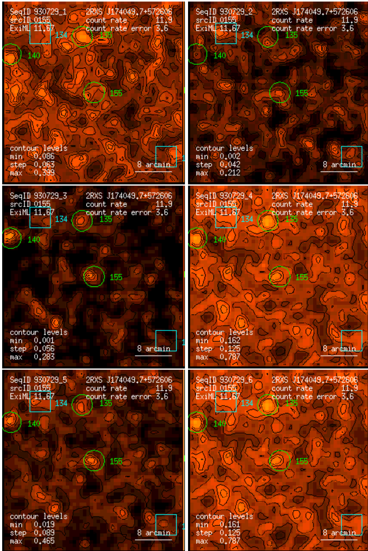
Figure 155: RASS 930729: detection 0155: band rate images, Gaussian filter: (1) PSPC channels 11 – 41, (2) 52 – 90, (3) 91 – 201, (4) 11 – 235, (5) 52 – 201, (6) 11 – 201. Broad band rates in counts/ks. Band rate contour levels in counts/ks/arcmin 2 .
