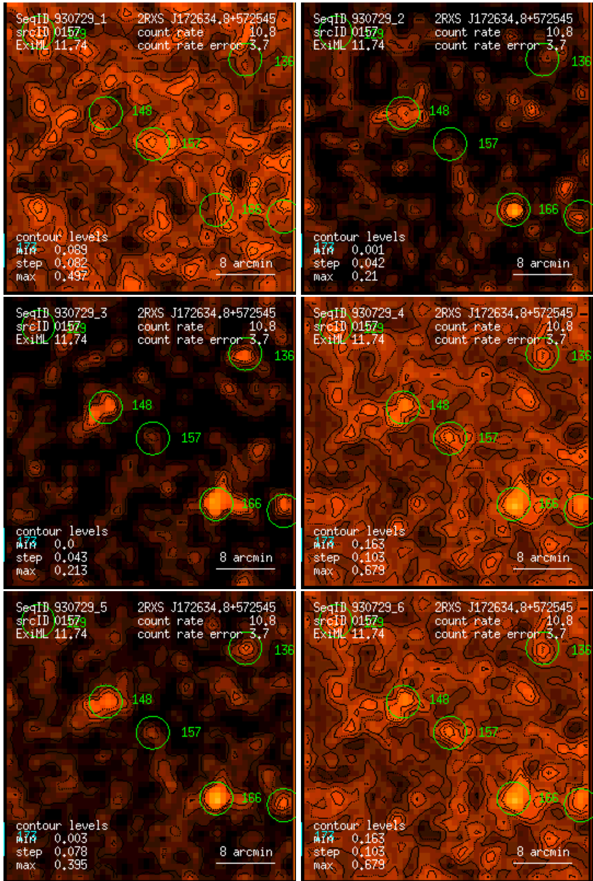
Figure 157: RASS 930729: detection 0157: band rate images, Gaussian filter: (1) PSPC channels 11 – 41, (2) 52 – 90, (3) 91 – 201, (4) 11 – 235, (5) 52 – 201, (6) 11 – 201. Broad band rates in counts/ks. Band rate contour levels in counts/ks/arcmin 2 .
