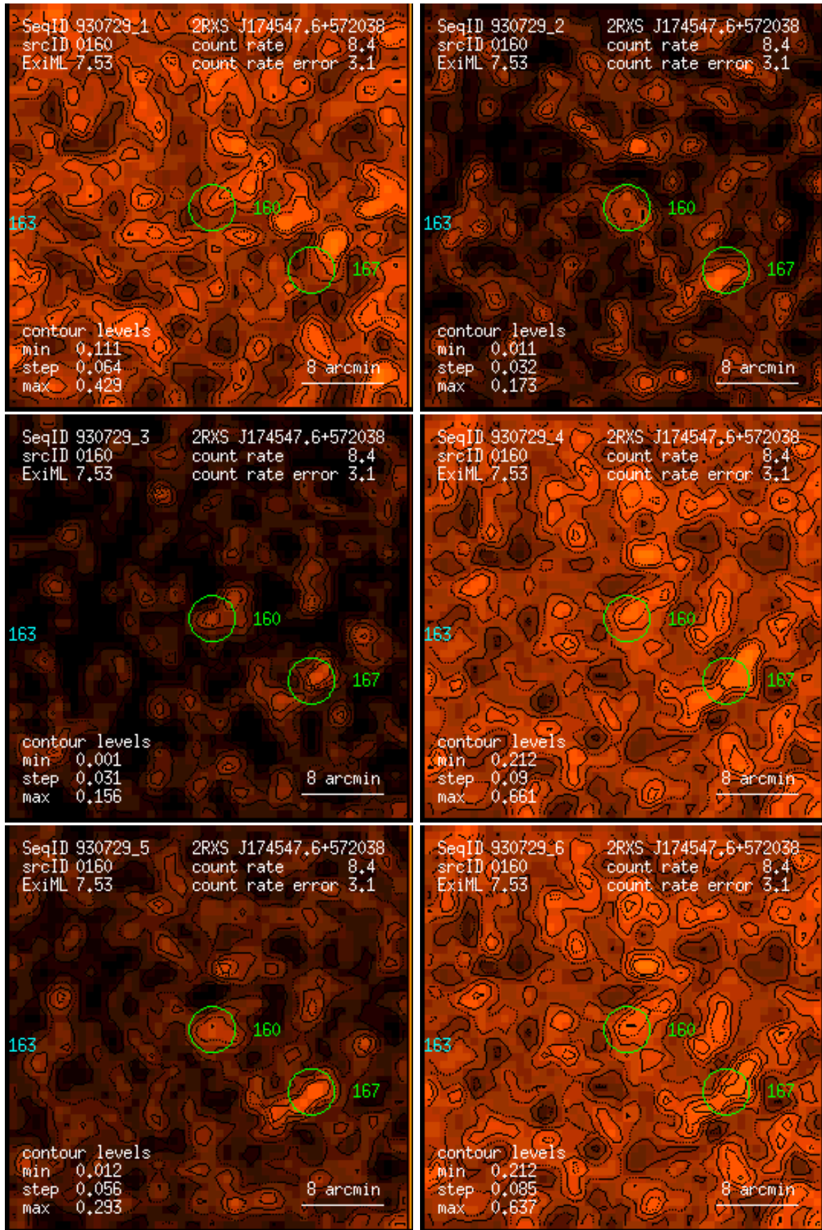
Figure 160: RASS 930729: detection 0160: band rate images, Gaussian filter: (1) PSPC channels 11 – 41, (2) 52 – 90, (3) 91 – 201, (4) 11 – 235, (5) 52 – 201, (6) 11 – 201. Broad band rates in counts/ks. Band rate contour levels in counts/ks/arcmin 2 .
