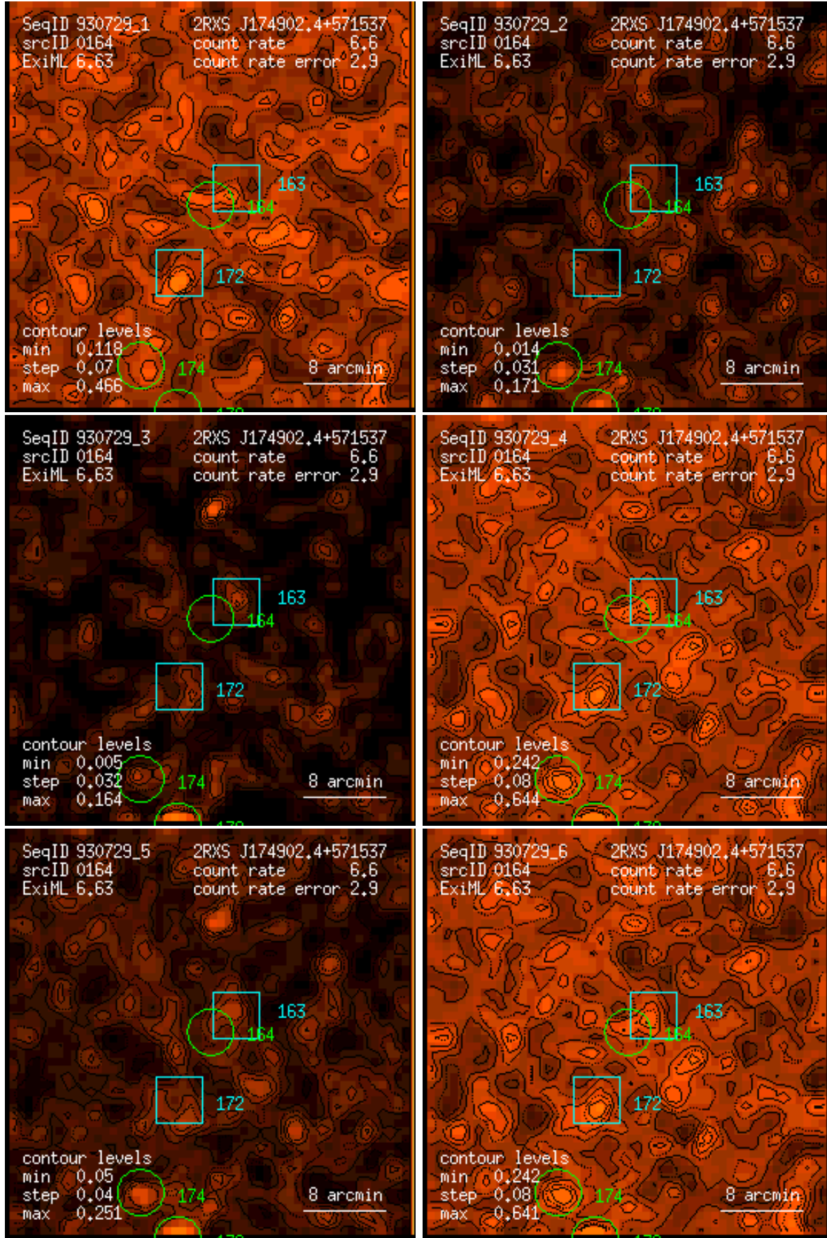
Figure 164: RASS 930729: detection 0164: band rate images, Gaussian filter: (1) PSPC channels 11 – 41, (2) 52 – 90, (3) 91 – 201, (4) 11 – 235, (5) 52 – 201, (6) 11 – 201. Broad band rates in counts/ks. Band rate contour levels in counts/ks/arcmin 2 .
