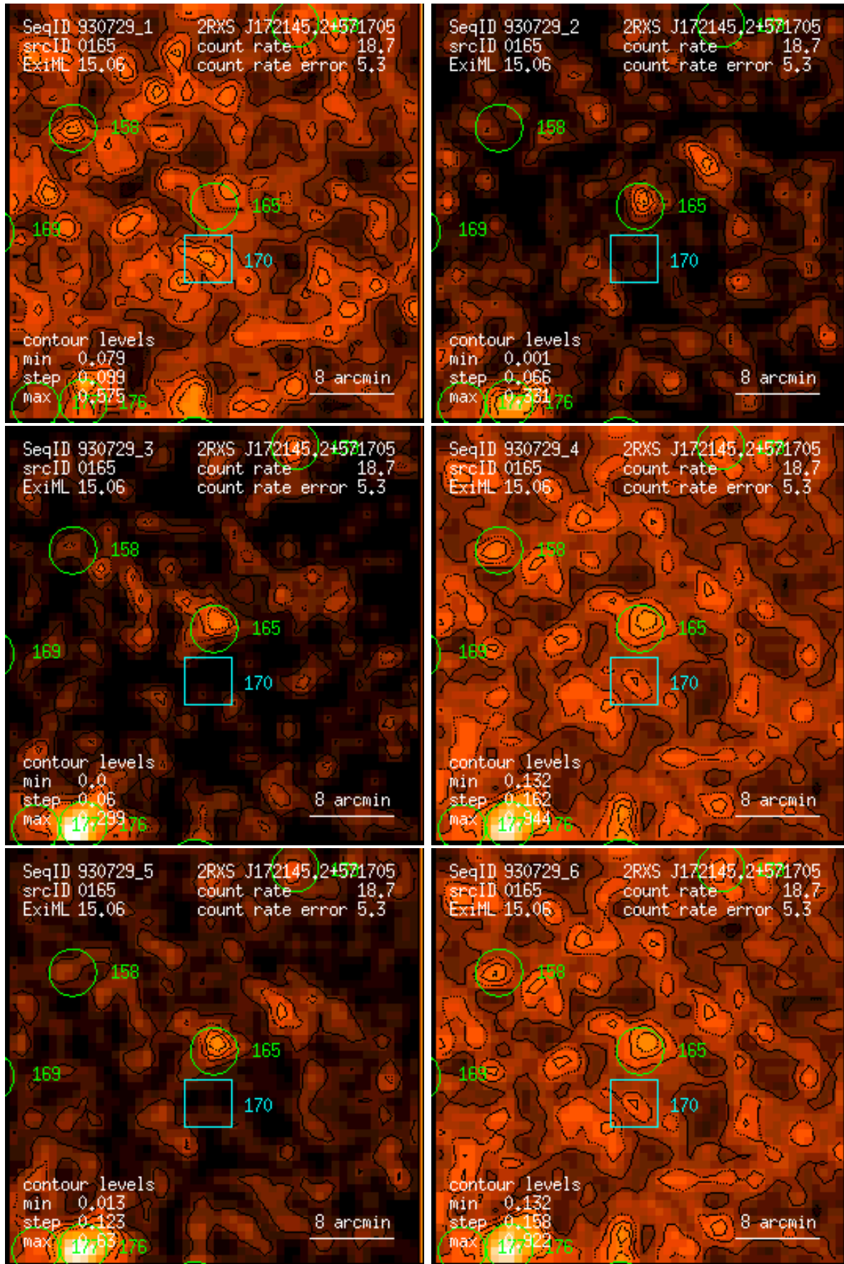
Figure 165: RASS 930729: detection 0165: band rate images, Gaussian filter: (1) PSPC channels 11 – 41, (2) 52 – 90, (3) 91 – 201, (4) 11 – 235, (5) 52 – 201, (6) 11 – 201. Broad band rates in counts/ks. Band rate contour levels in counts/ks/arcmin 2 .
