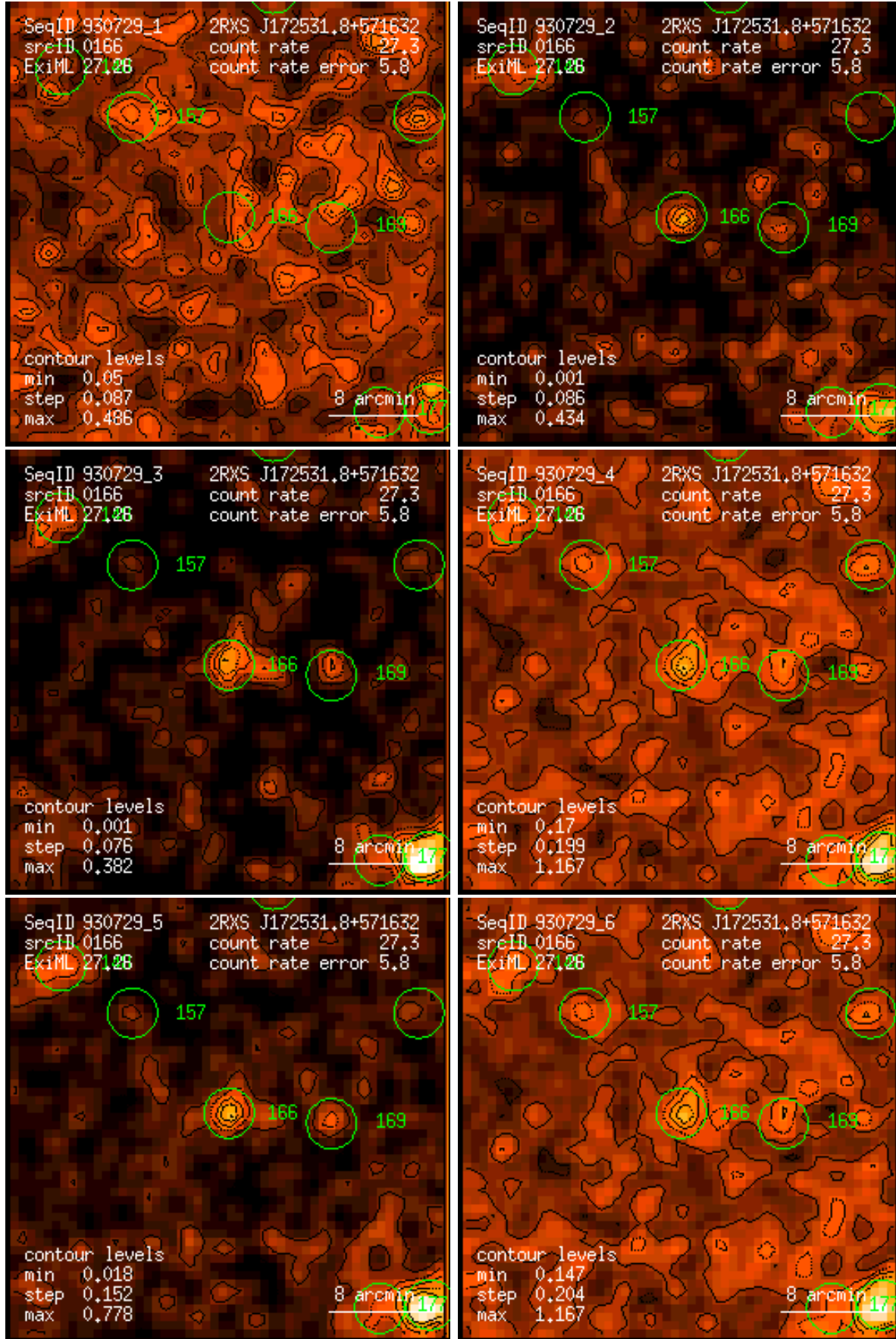
Figure 166: RASS 930729: detection 0166: band rate images, Gaussian filter: (1) PSPC channels 11 – 41, (2) 52 – 90, (3) 91 – 201, (4) 11 – 235, (5) 52 – 201, (6) 11 – 201. Broad band rates in counts/ks. Band rate contour levels in counts/ks/arcmin 2 .
