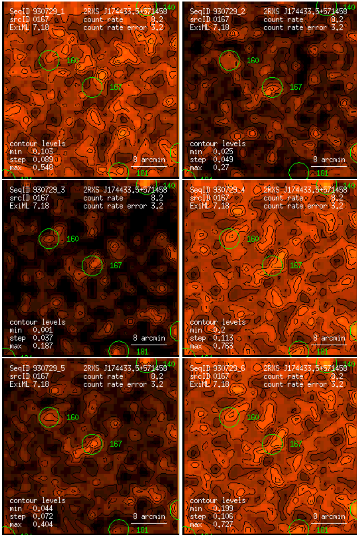
Figure 167: RASS 930729: detection 0167: band rate images, Gaussian filter: (1) PSPC channels 11 – 41, (2) 52 – 90, (3) 91 – 201, (4) 11 – 235, (5) 52 – 201, (6) 11 – 201. Broad band rates in counts/ks. Band rate contour levels in counts/ks/arcmin 2 .
