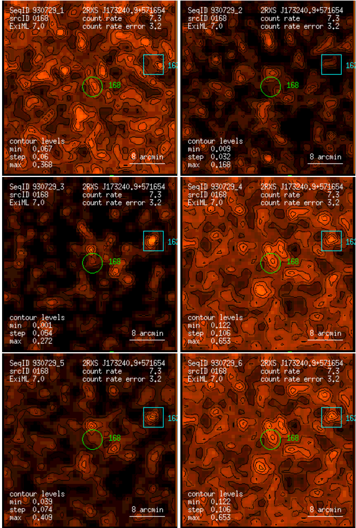
Figure 168: RASS 930729: detection 0168: band rate images, Gaussian filter: (1) PSPC channels 11 – 41, (2) 52 – 90, (3) 91 – 201, (4) 11 – 235, (5) 52 – 201, (6) 11 – 201. Broad band rates in counts/ks. Band rate contour levels in counts/ks/arcmin 2 .
