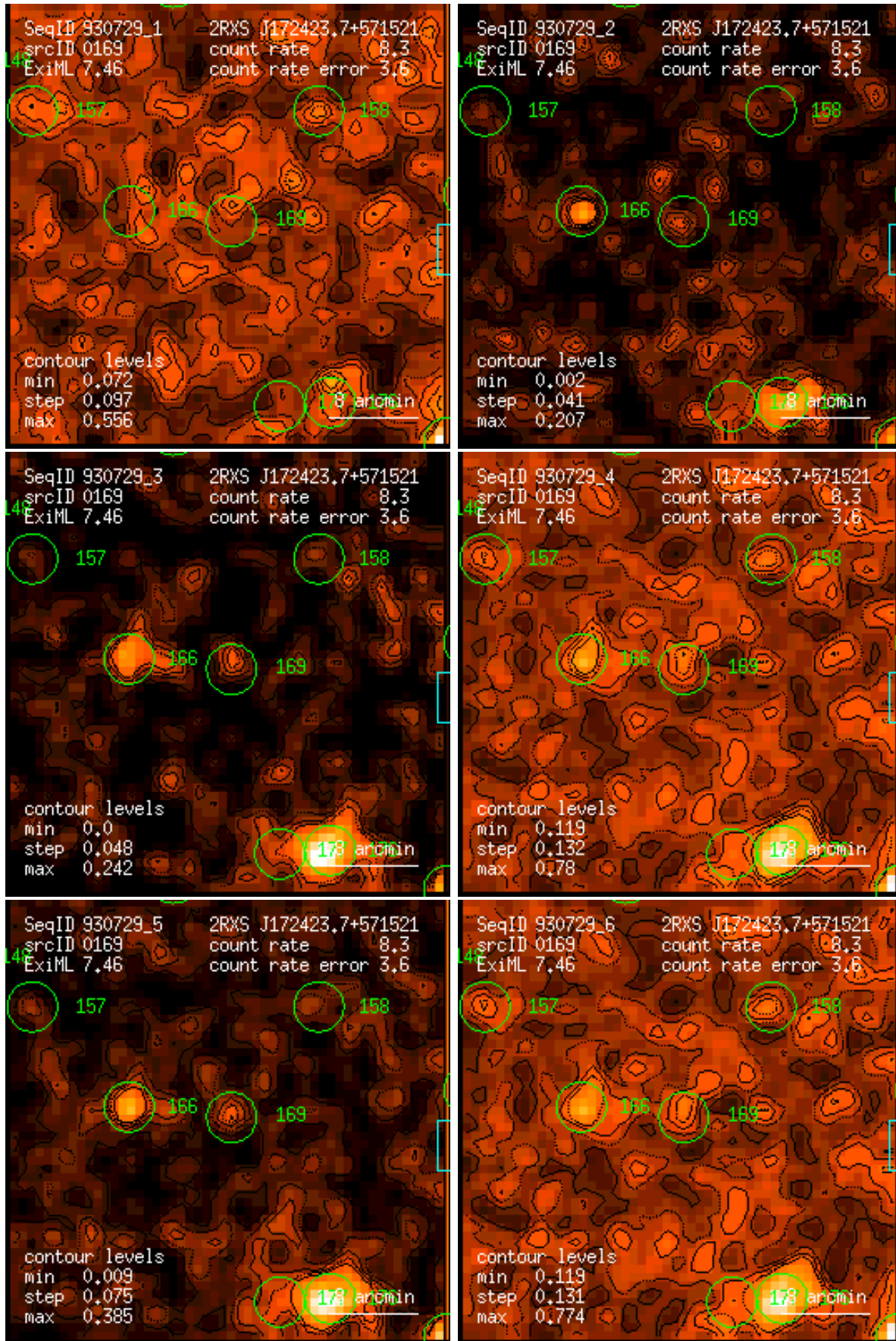
Figure 169: RASS 930729: detection 0169: band rate images, Gaussian filter: (1) PSPC channels 11 – 41, (2) 52 – 90, (3) 91 – 201, (4) 11 – 235, (5) 52 – 201, (6) 11 – 201. Broad band rates in counts/ks. Band rate contour levels in counts/ks/arcmin 2 .
