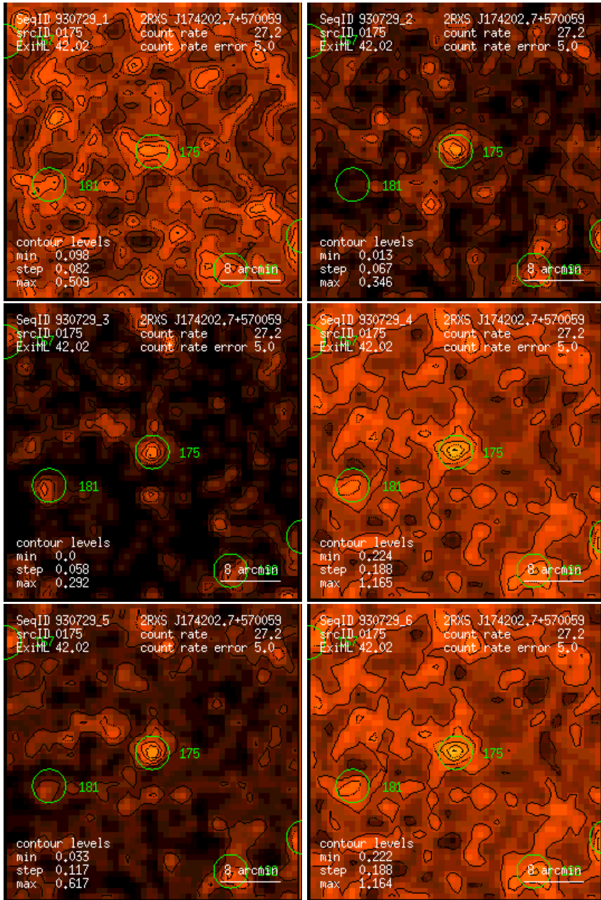
Figure 175: RASS 930729: detection 0175: band rate images, Gaussian filter: (1) PSPC channels 11 – 41, (2) 52 – 90, (3) 91 – 201, (4) 11 – 235, (5) 52 – 201, (6) 11 – 201. Broad band rates in counts/ks. Band rate contour levels in counts/ks/arcmin 2 .
