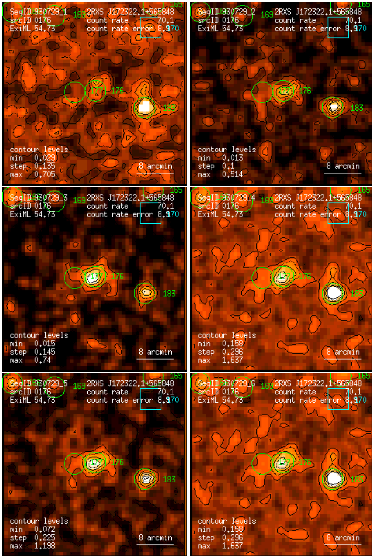
Figure 176: RASS 930729: detection 0176: band rate images, Gaussian filter: (1) PSPC channels 11 – 41, (2) 52 – 90, (3) 91 – 201, (4) 11 – 235, (5) 52 – 201, (6) 11 – 201. Broad band rates in counts/ks. Band rate contour levels in counts/ks/arcmin 2 .
