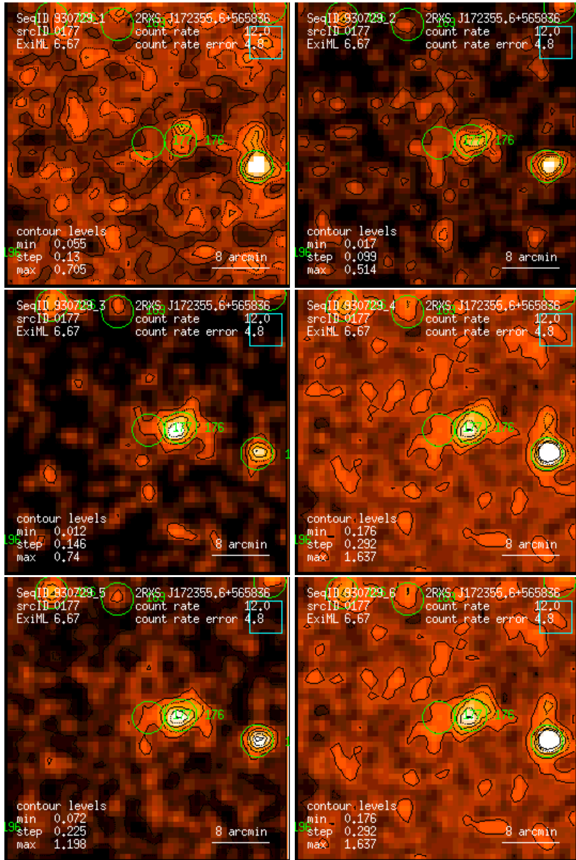
Figure 177: RASS 930729: detection 0177: band rate images, Gaussian filter: (1) PSPC channels 11 – 41, (2) 52 – 90, (3) 91 – 201, (4) 11 – 235, (5) 52 – 201, (6) 11 – 201. Broad band rates in counts/ks. Band rate contour levels in counts/ks/arcmin 2 .
