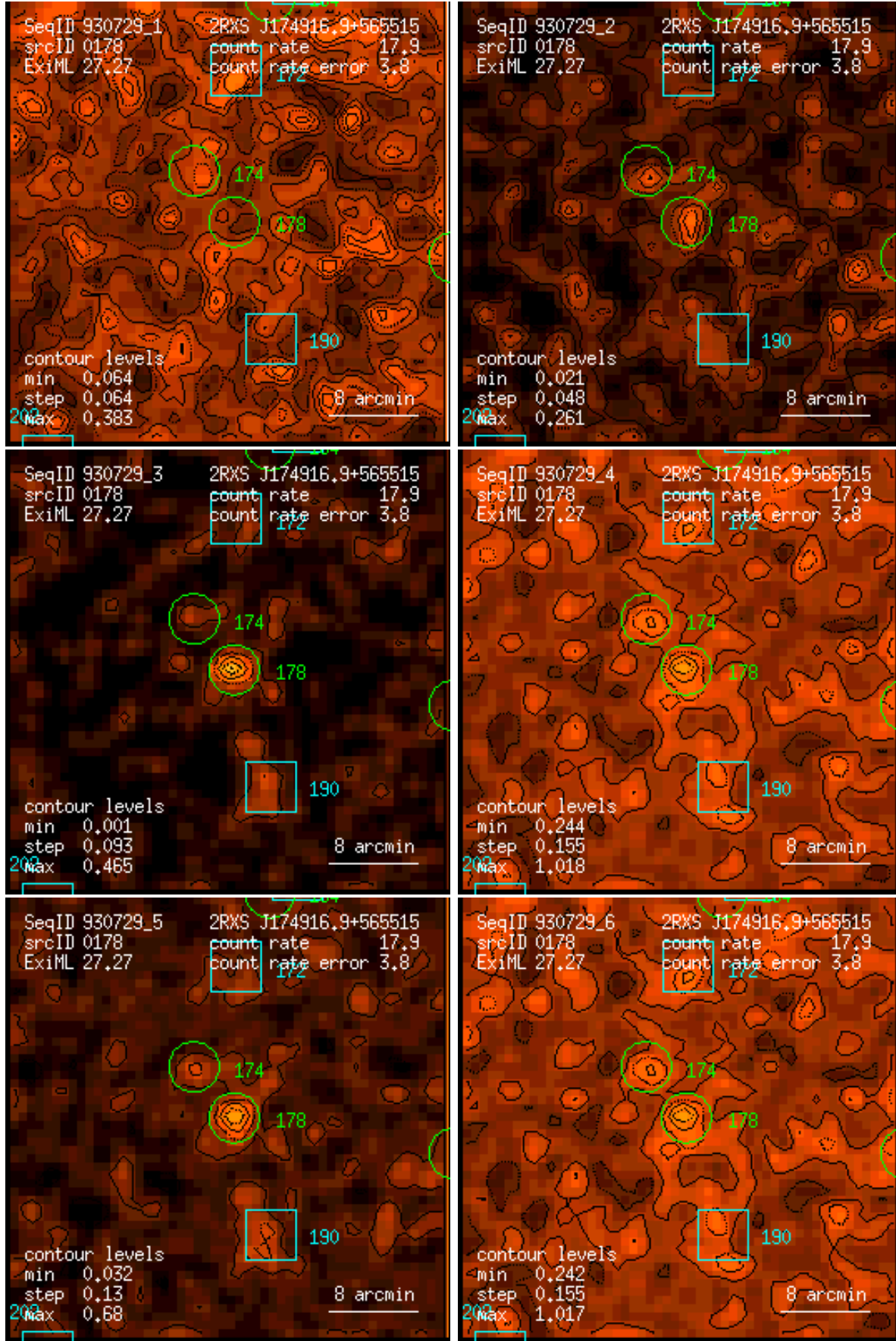
Figure 178: RASS 930729: detection 0178: band rate images, Gaussian filter: (1) PSPC channels 11 – 41, (2) 52 – 90, (3) 91 – 201, (4) 11 – 235, (5) 52 – 201, (6) 11 – 201. Broad band rates in counts/ks. Band rate contour levels in counts/ks/arcmin 2 .
