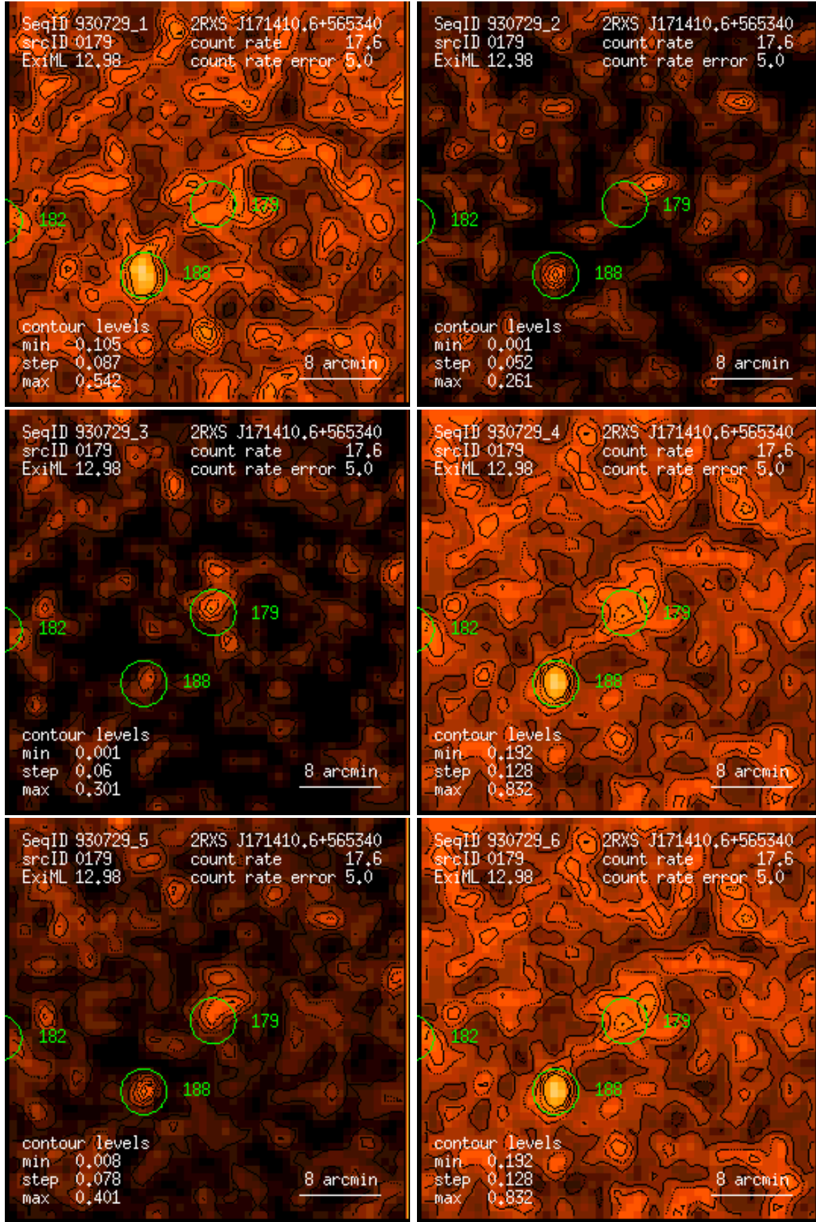
Figure 179: RASS 930729: detection 0179: band rate images, Gaussian filter: (1) PSPC channels 11 – 41, (2) 52 – 90, (3) 91 – 201, (4) 11 – 235, (5) 52 – 201, (6) 11 – 201. Broad band rates in counts/ks. Band rate contour levels in counts/ks/arcmin 2 .
