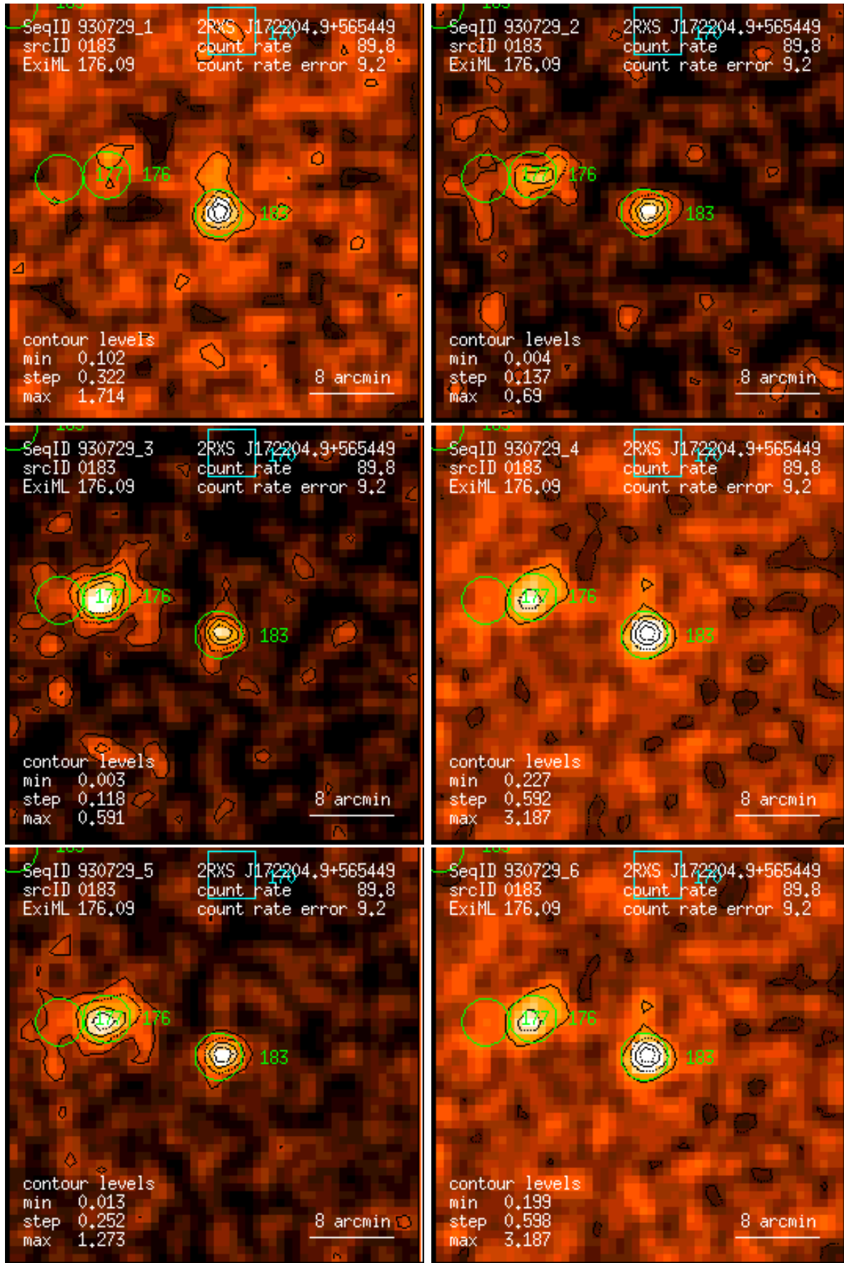
Figure 183: RASS 930729: detection 0183: band rate images, Gaussian filter: (1) PSPC channels 11 – 41, (2) 52 – 90, (3) 91 – 201, (4) 11 – 235, (5) 52 – 201, (6) 11 – 201. Broad band rates in counts/ks. Band rate contour levels in counts/ks/arcmin 2 .
