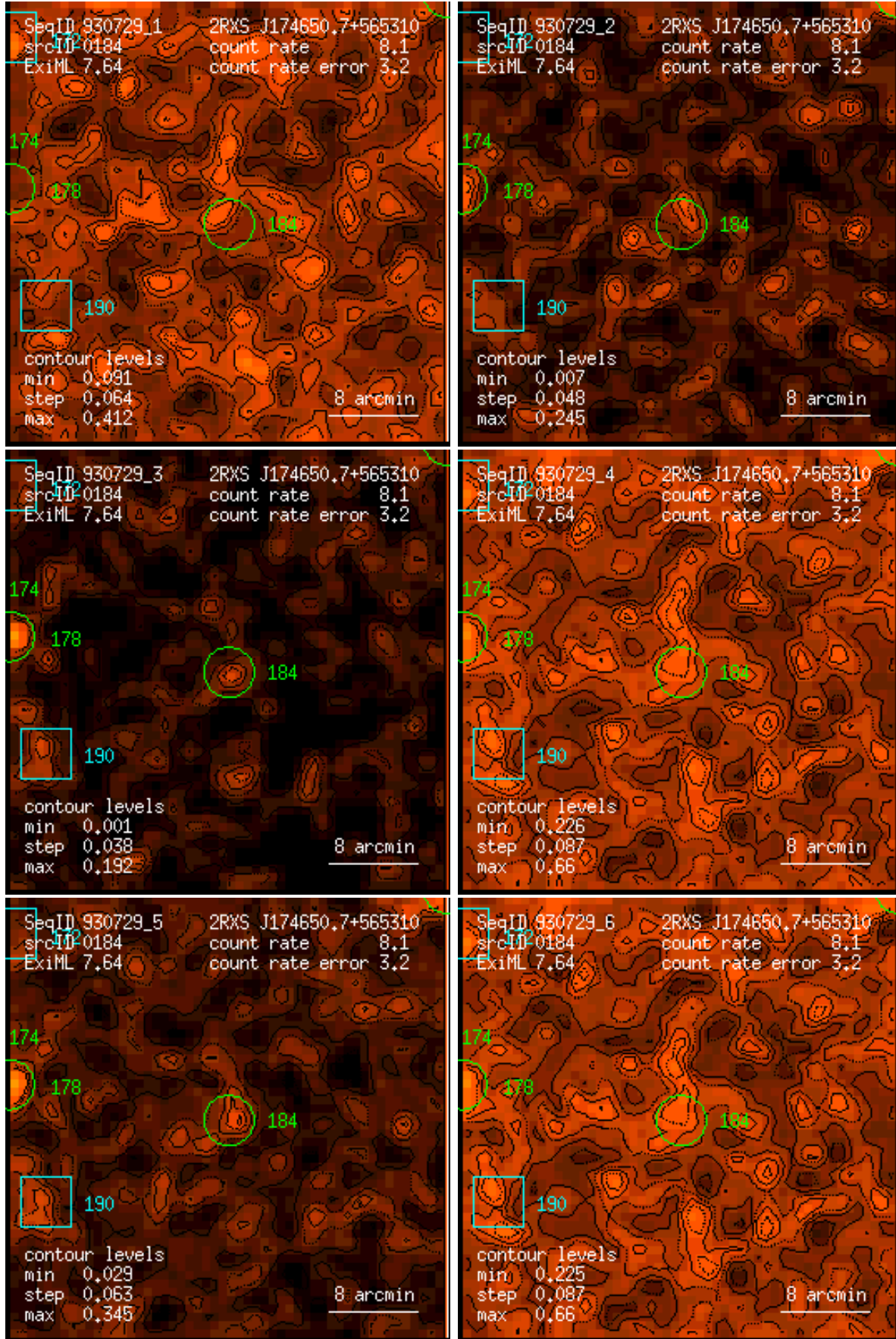
Figure 184: RASS 930729: detection 0184: band rate images, Gaussian filter: (1) PSPC channels 11 – 41, (2) 52 – 90, (3) 91 – 201, (4) 11 – 235, (5) 52 – 201, (6) 11 – 201. Broad band rates in counts/ks. Band rate contour levels in counts/ks/arcmin 2 .
