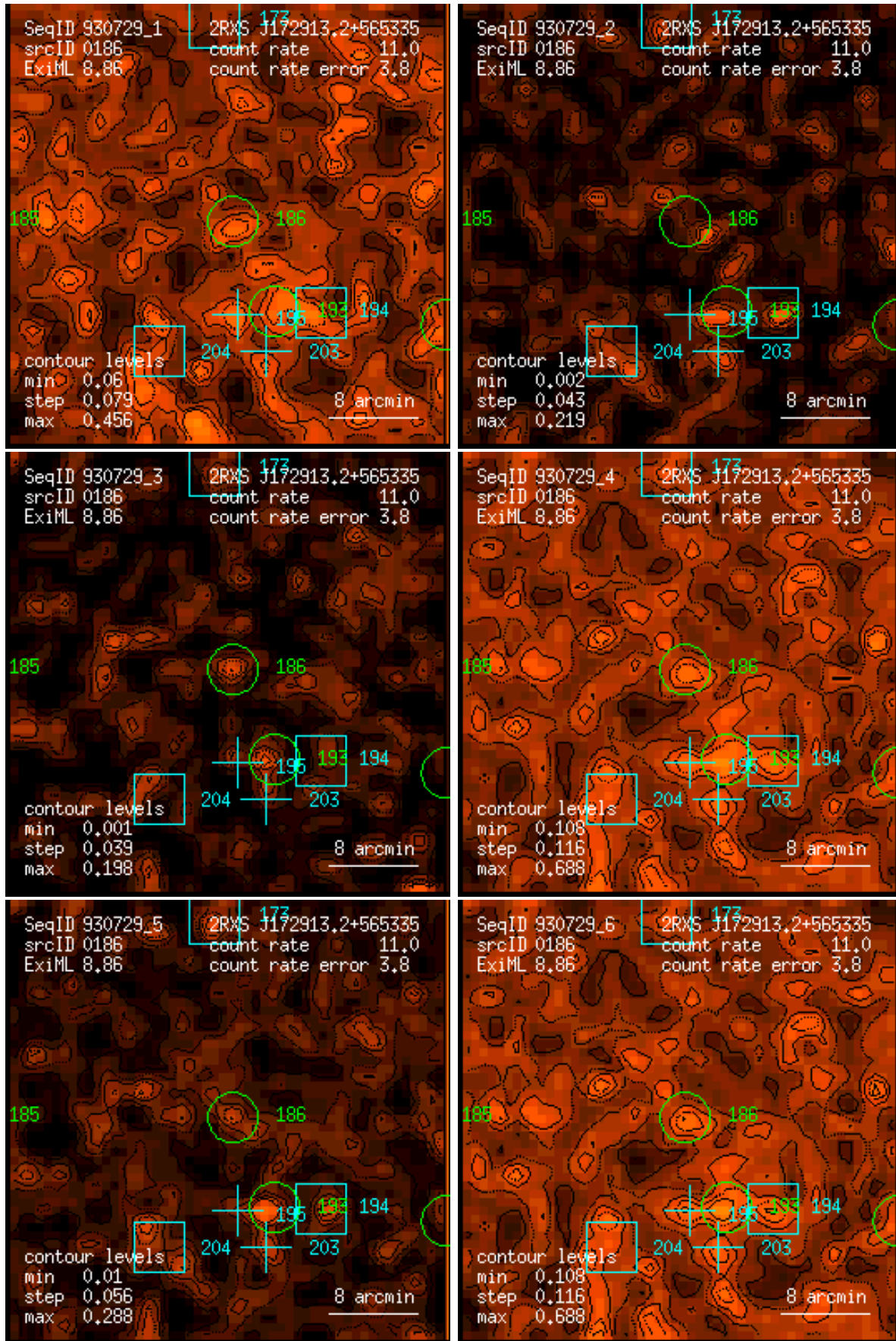
Figure 186: RASS 930729: detection 0186: band rate images, Gaussian filter: (1) PSPC channels 11 – 41, (2) 52 – 90, (3) 91 – 201, (4) 11 – 235, (5) 52 – 201, (6) 11 – 201. Broad band rates in counts/ks. Band rate contour levels in counts/ks/arcmin 2 .
