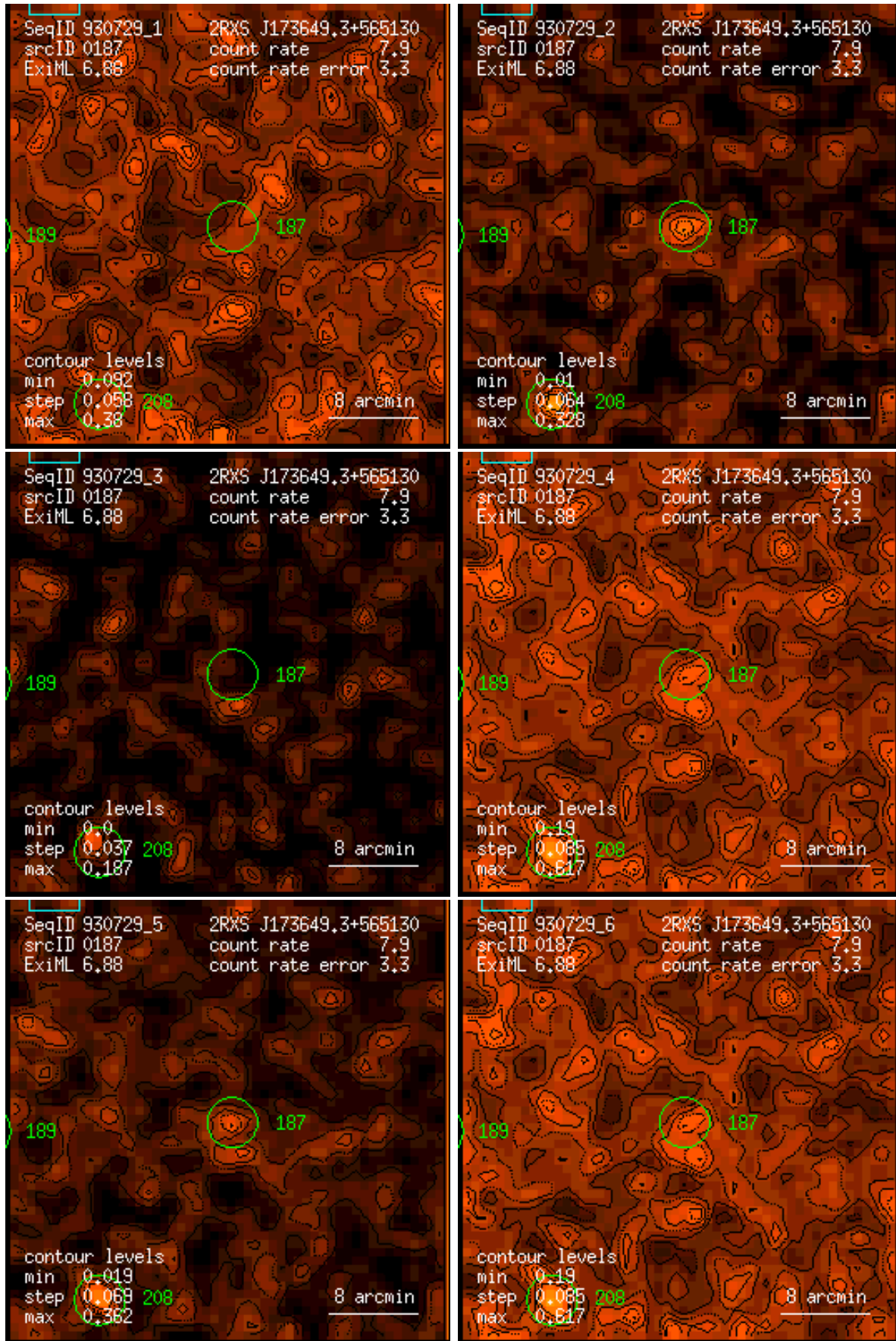
Figure 187: RASS 930729: detection 0187: band rate images, Gaussian filter: (1) PSPC channels 11 – 41, (2) 52 – 90, (3) 91 – 201, (4) 11 – 235, (5) 52 – 201, (6) 11 – 201. Broad band rates in counts/ks. Band rate contour levels in counts/ks/arcmin 2 .
