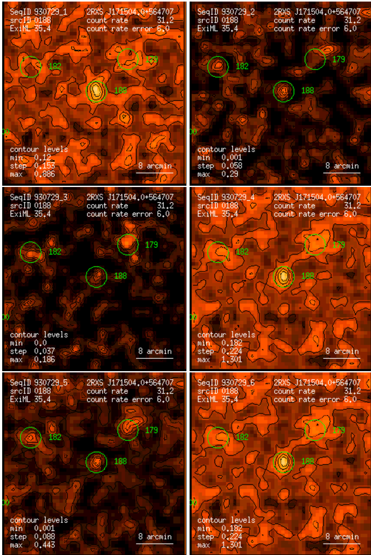
Figure 188: RASS 930729: detection 0188: band rate images, Gaussian filter: (1) PSPC channels 11 – 41, (2) 52 – 90, (3) 91 – 201, (4) 11 – 235, (5) 52 – 201, (6) 11 – 201. Broad band rates in counts/ks. Band rate contour levels in counts/ks/arcmin 2 .
