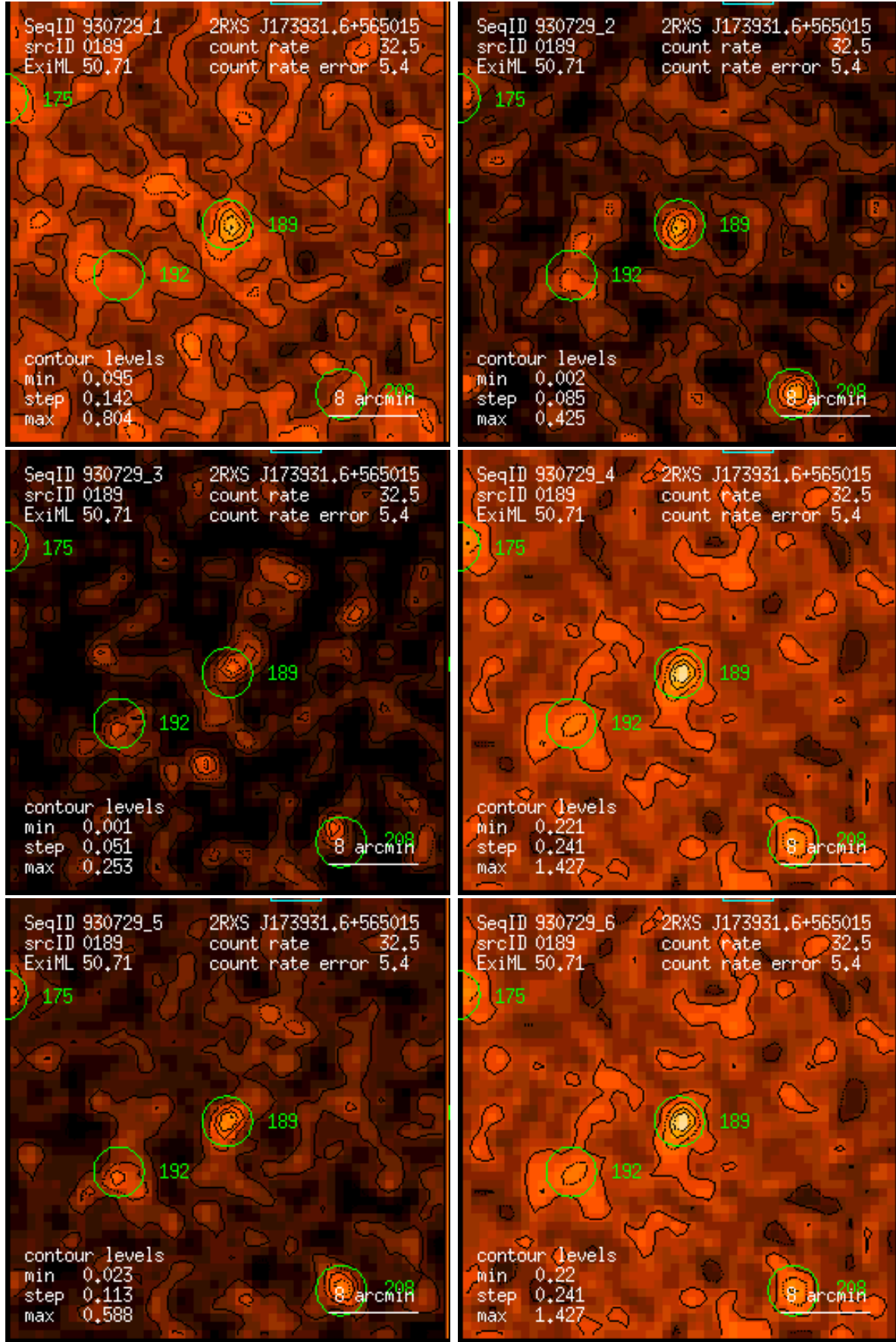
Figure 189: RASS 930729: detection 0189: band rate images, Gaussian filter: (1) PSPC channels 11 – 41, (2) 52 – 90, (3) 91 – 201, (4) 11 – 235, (5) 52 – 201, (6) 11 – 201. Broad band rates in counts/ks. Band rate contour levels in counts/ks/arcmin 2 .
