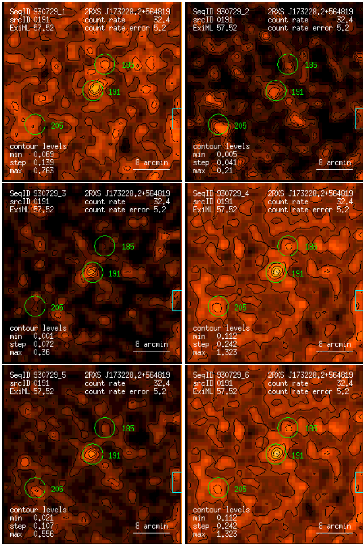
Figure 191: RASS 930729: detection 0191: band rate images, Gaussian filter: (1) PSPC channels 11 – 41, (2) 52 – 90, (3) 91 – 201, (4) 11 – 235, (5) 52 – 201, (6) 11 – 201. Broad band rates in counts/ks. Band rate contour levels in counts/ks/arcmin 2 .
