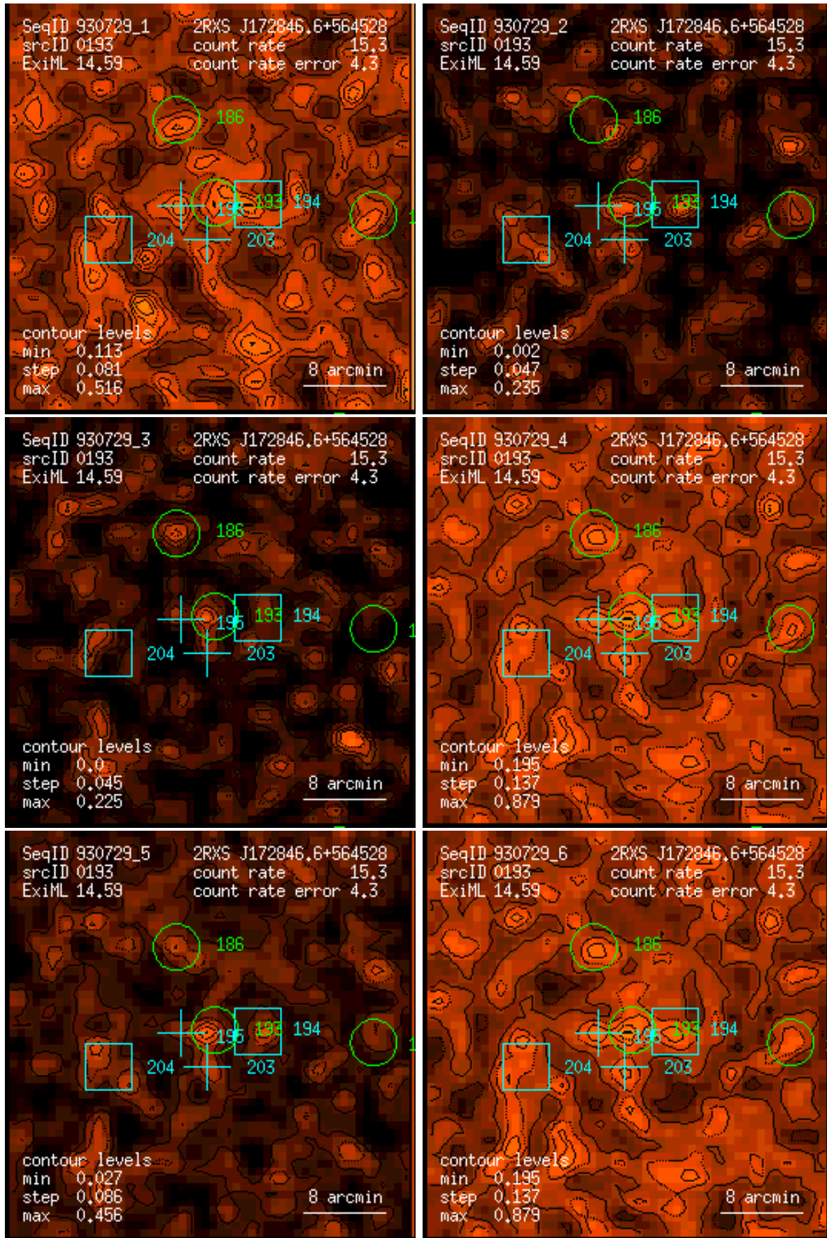
Figure 193: RASS 930729: detection 0193: band rate images, Gaussian filter: (1) PSPC channels 11 – 41, (2) 52 – 90, (3) 91 – 201, (4) 11 – 235, (5) 52 – 201, (6) 11 – 201. Broad band rates in counts/ks. Band rate contour levels in counts/ks/arcmin 2 .
