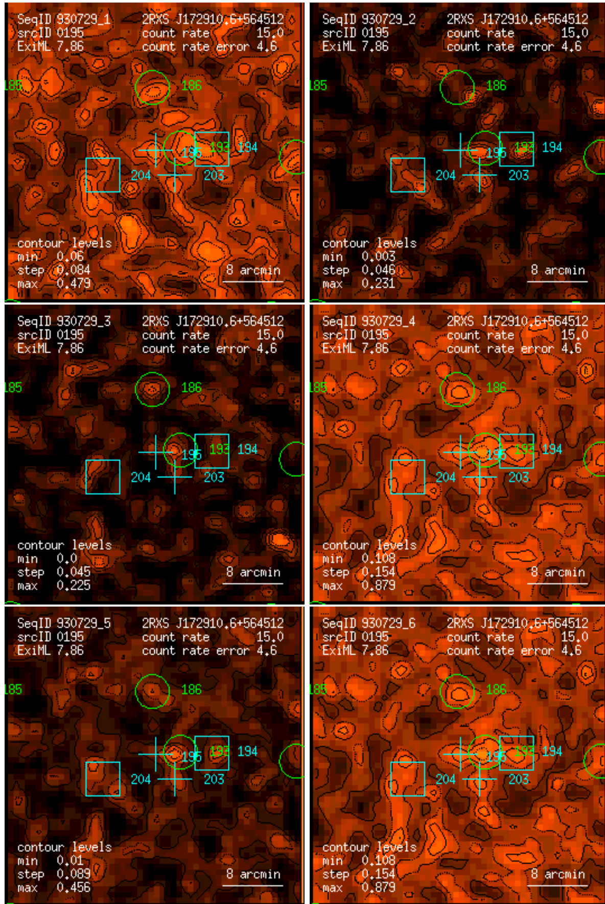
Figure 195: RASS 930729: detection 0195: band rate images, Gaussian filter: (1) PSPC channels 11 – 41, (2) 52 – 90, (3) 91 – 201, (4) 11 – 235, (5) 52 – 201, (6) 11 – 201. Broad band rates in counts/ks. Band rate contour levels in counts/ks/arcmin 2 .
