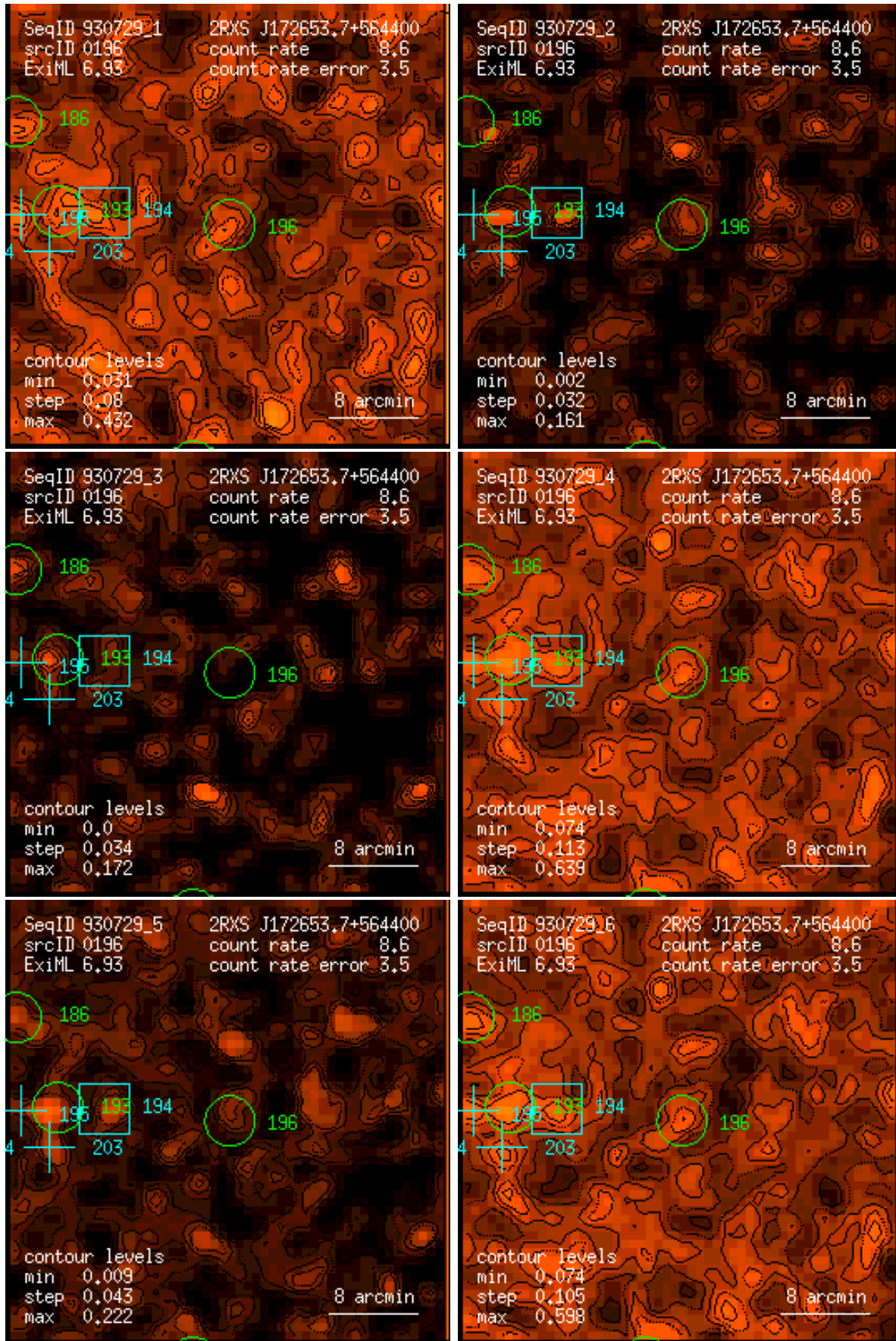
Figure 196: RASS 930729: detection 0196: band rate images, Gaussian filter: (1) PSPC channels 11 – 41, (2) 52 – 90, (3) 91 – 201, (4) 11 – 235, (5) 52 – 201, (6) 11 – 201. Broad band rates in counts/ks. Band rate contour levels in counts/ks/arcmin 2 .
