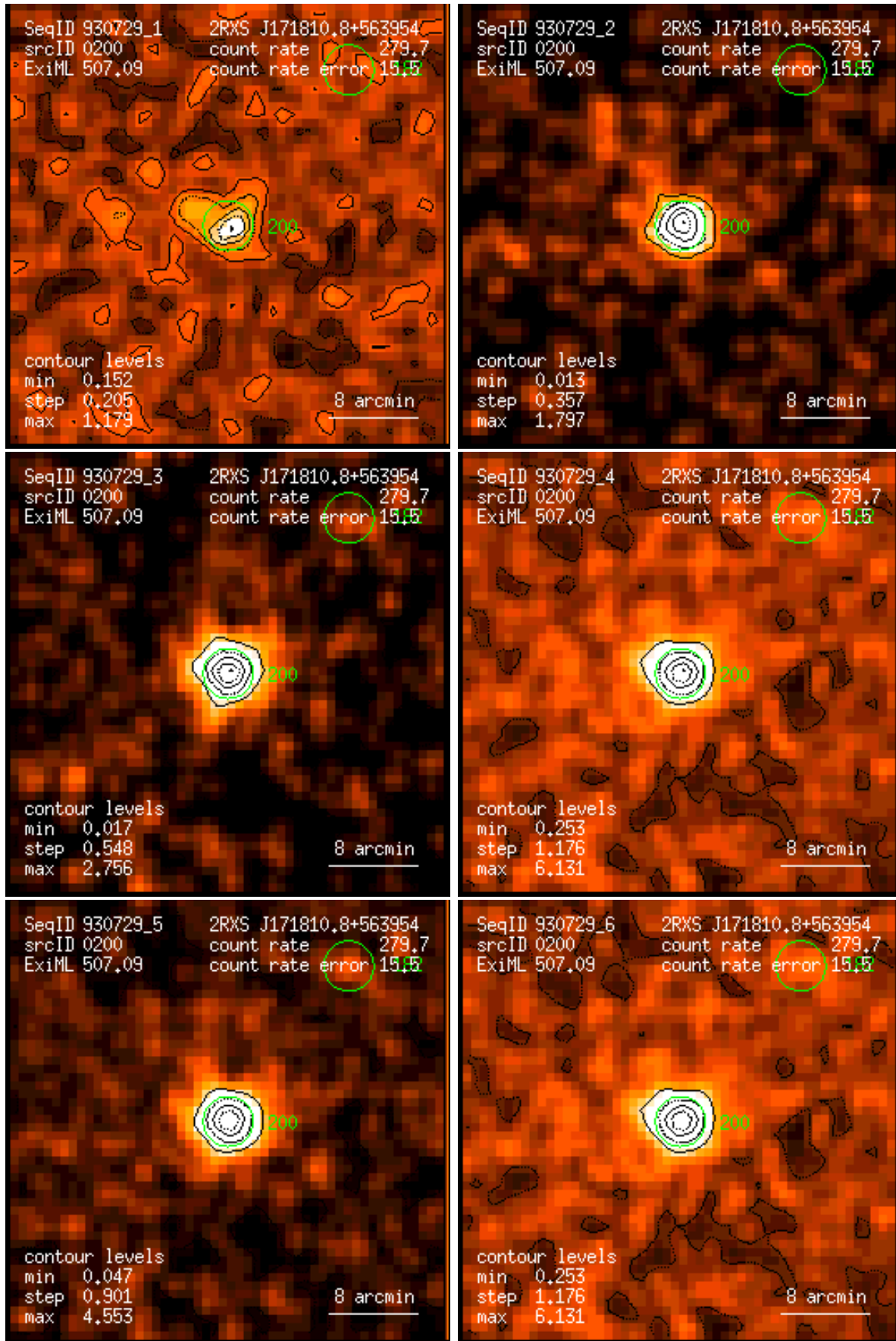
Figure 200: RASS 930729: detection 0200: band rate images, Gaussian filter: (1) PSPC channels 11 – 41, (2) 52 – 90, (3) 91 – 201, (4) 11 – 235, (5) 52 – 201, (6) 11 – 201. Broad band rates in counts/ks. Band rate contour levels in counts/ks/arcmin 2 .
