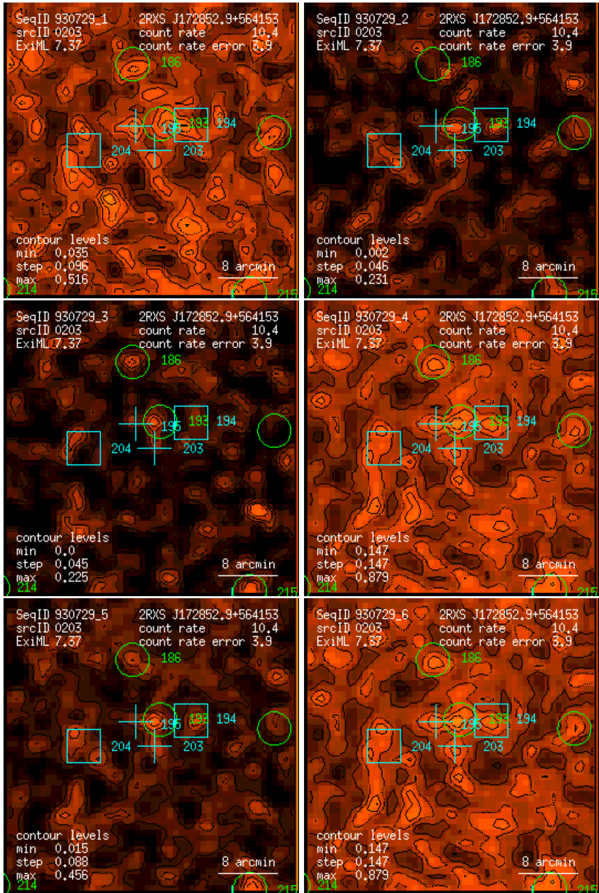
Figure 203: RASS 930729: detection 0203: band rate images, Gaussian filter: (1) PSPC channels 11 – 41, (2) 52 – 90, (3) 91 – 201, (4) 11 – 235, (5) 52 – 201, (6) 11 – 201. Broad band rates in counts/ks. Band rate contour levels in counts/ks/arcmin 2 .
