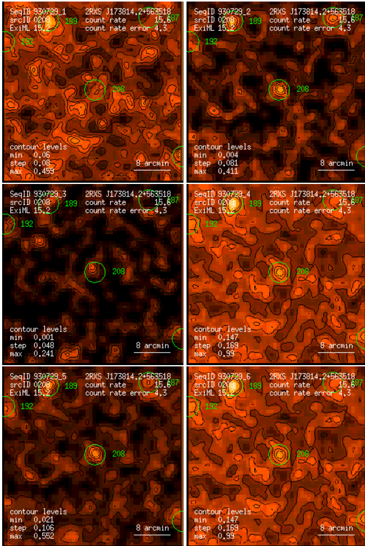
Figure 208: RASS 930729: detection 0208: band rate images, Gaussian filter: (1) PSPC channels 11 – 41, (2) 52 – 90, (3) 91 – 201, (4) 11 – 235, (5) 52 – 201, (6) 11 – 201. Broad band rates in counts/ks. Band rate contour levels in counts/ks/arcmin 2 .
