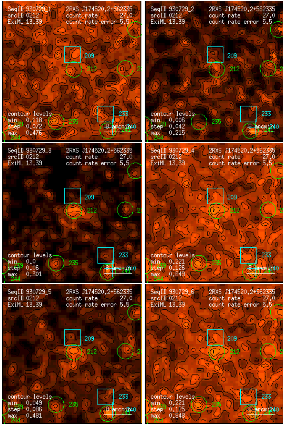
Figure 212: RASS 930729: detection 0212: band rate images, Gaussian filter: (1) PSPC channels 11 – 41, (2) 52 – 90, (3) 91 – 201, (4) 11 – 235, (5) 52 – 201, (6) 11 – 201. Broad band rates in counts/ks. Band rate contour levels in counts/ks/arcmin 2 .
