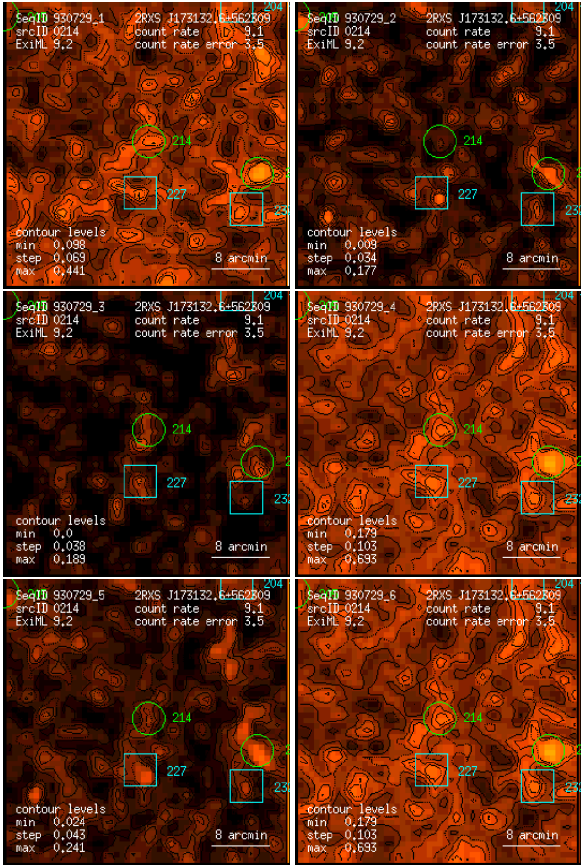
Figure 214: RASS 930729: detection 0214: band rate images, Gaussian filter: (1) PSPC channels 11 – 41, (2) 52 – 90, (3) 91 – 201, (4) 11 – 235, (5) 52 – 201, (6) 11 – 201. Broad band rates in counts/ks. Band rate contour levels in counts/ks/arcmin 2 .
