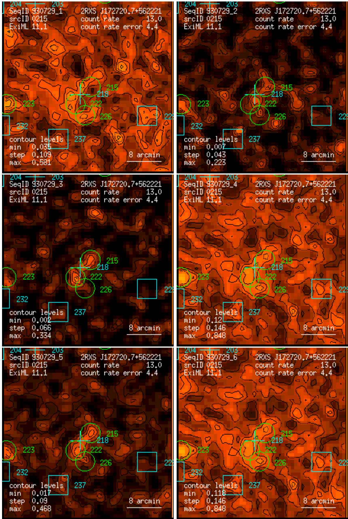
Figure 215: RASS 930729: detection 0215: band rate images, Gaussian filter: (1) PSPC channels 11 – 41, (2) 52 – 90, (3) 91 – 201, (4) 11 – 235, (5) 52 – 201, (6) 11 – 201. Broad band rates in counts/ks. Band rate contour levels in counts/ks/arcmin 2 .
