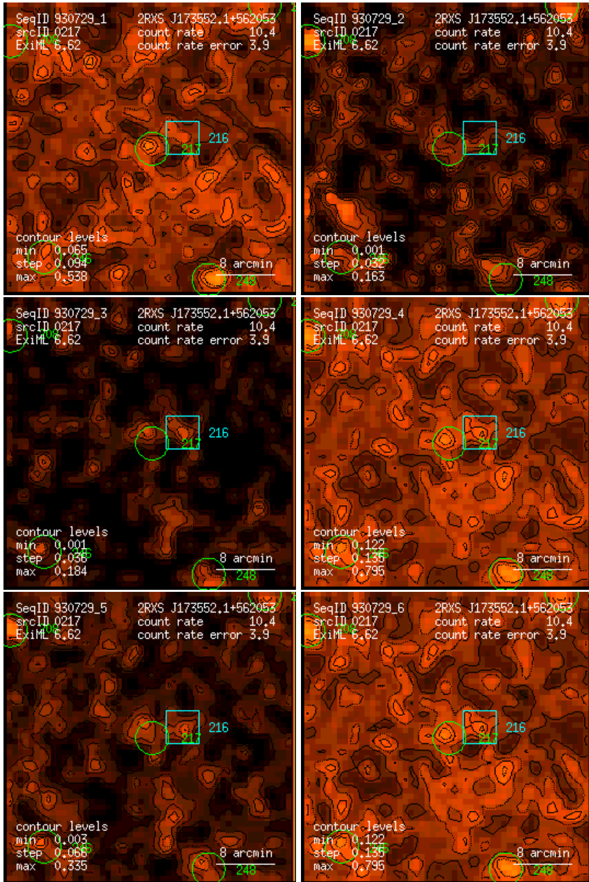
Figure 217: RASS 930729: detection 0217: band rate images, Gaussian filter: (1) PSPC channels 11 – 41, (2) 52 – 90, (3) 91 – 201, (4) 11 – 235, (5) 52 – 201, (6) 11 – 201. Broad band rates in counts/ks. Band rate contour levels in counts/ks/arcmin 2 .
