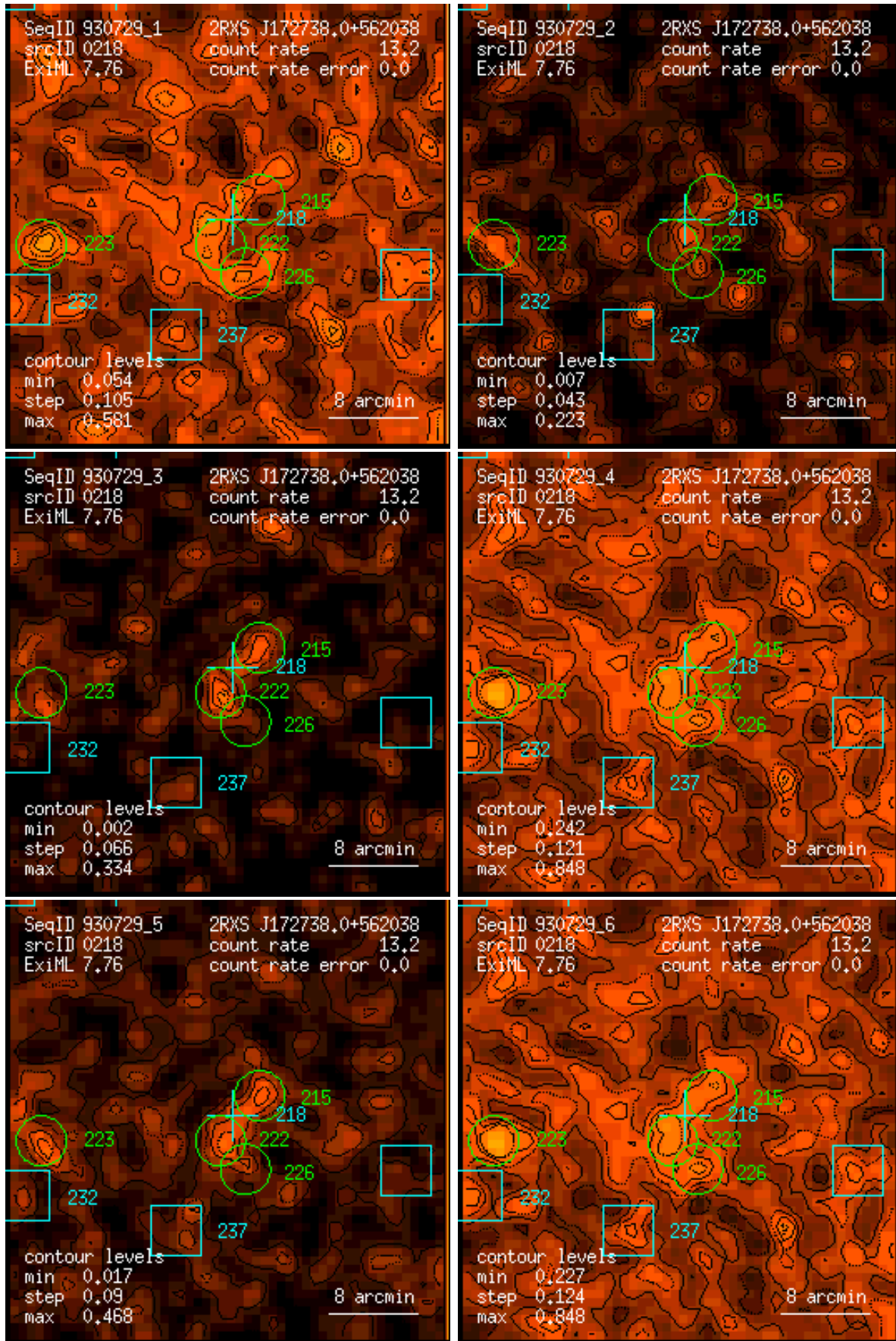
Figure 218: RASS 930729: detection 0218: band rate images, Gaussian filter: (1) PSPC channels 11 – 41, (2) 52 – 90, (3) 91 – 201, (4) 11 – 235, (5) 52 – 201, (6) 11 – 201. Broad band rates in counts/ks. Band rate contour levels in counts/ks/arcmin 2 .
