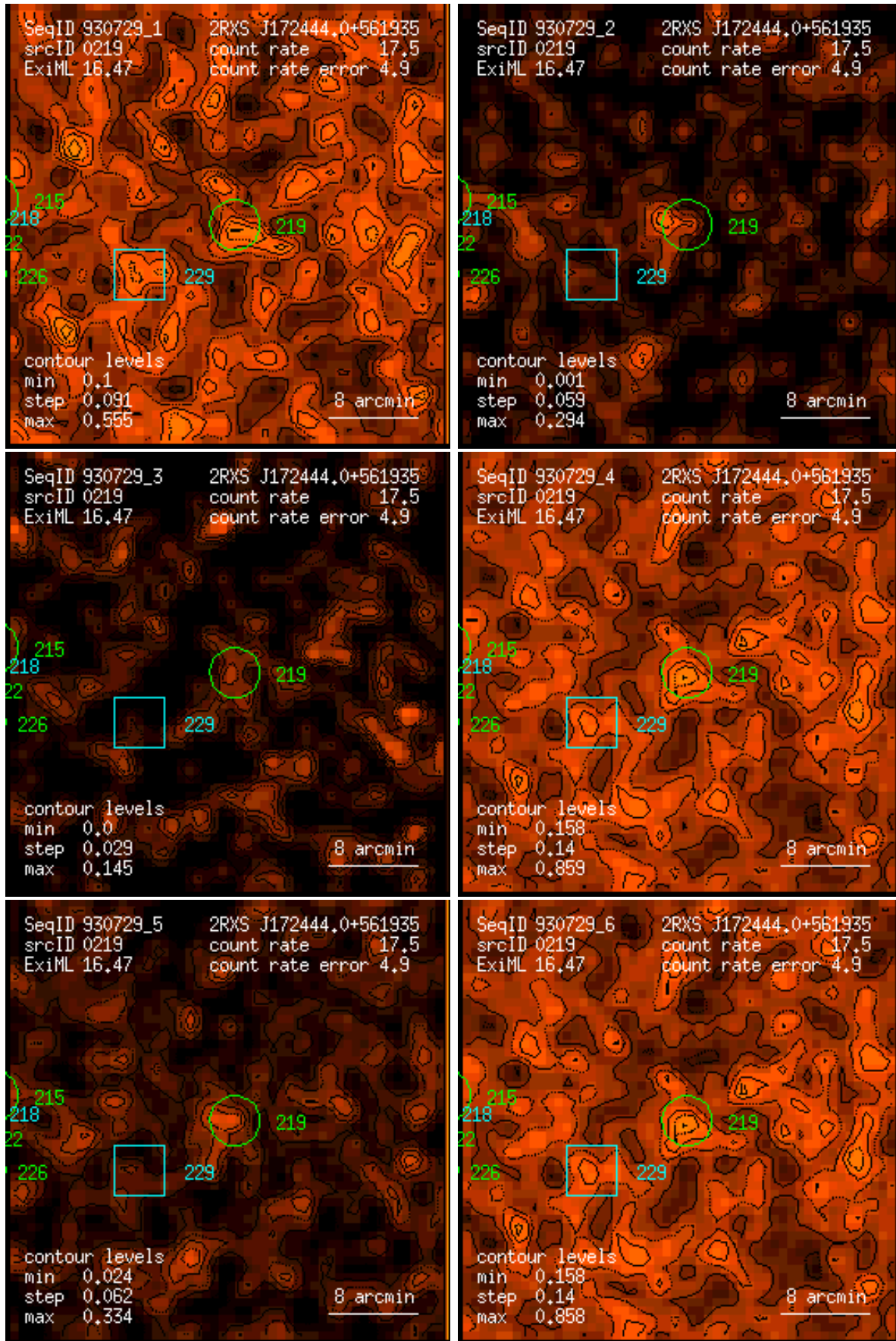
Figure 219: RASS 930729: detection 0219: band rate images, Gaussian filter: (1) PSPC channels 11 – 41, (2) 52 – 90, (3) 91 – 201, (4) 11 – 235, (5) 52 – 201, (6) 11 – 201. Broad band rates in counts/ks. Band rate contour levels in counts/ks/arcmin 2 .
